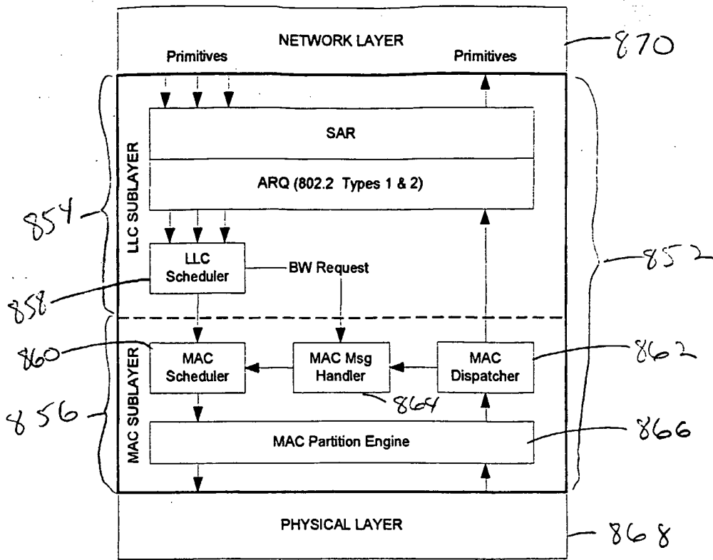
Figure 84. DLL layer components
