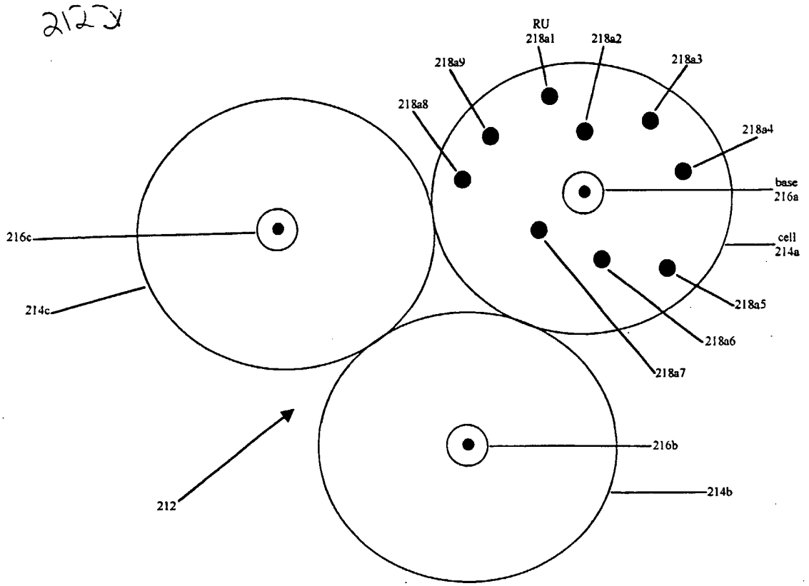
Figure 19. Network with base units and RUs.
