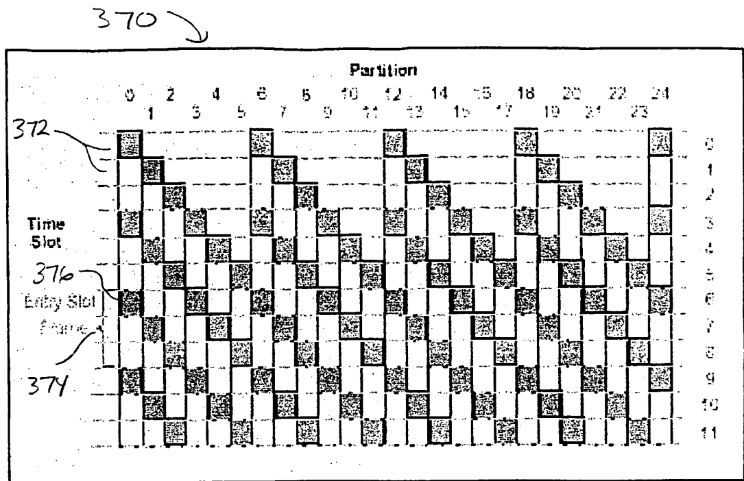
Figure 27. Partition layout for a lower subband with a spectral spreading factor of 2; 8 \times 3 + 1 layout; three timeslots per frame.
