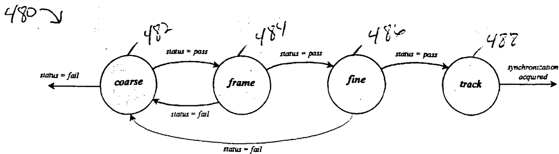
Figure 39. Synchronization Acquisition State Diagram.
