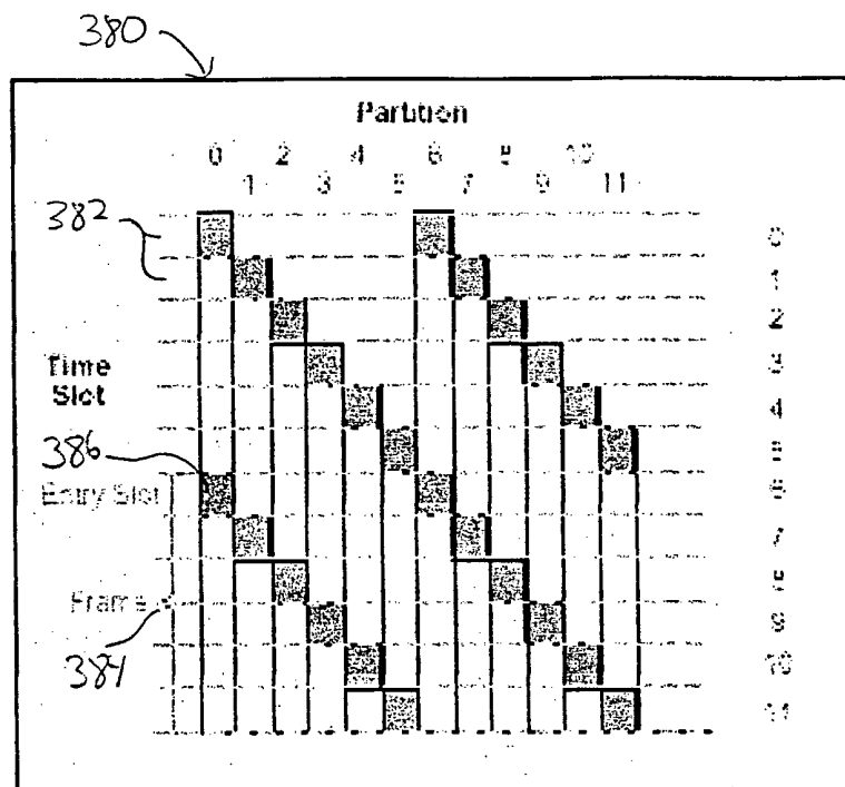
Figure 28. Partition layout for a lower subband with a spectral spreading factor of 4; a 2 \times 6 layout; six time slots per frame.
