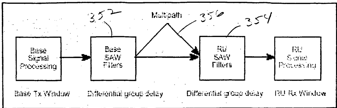
Figure 25. Guard Time Factors
