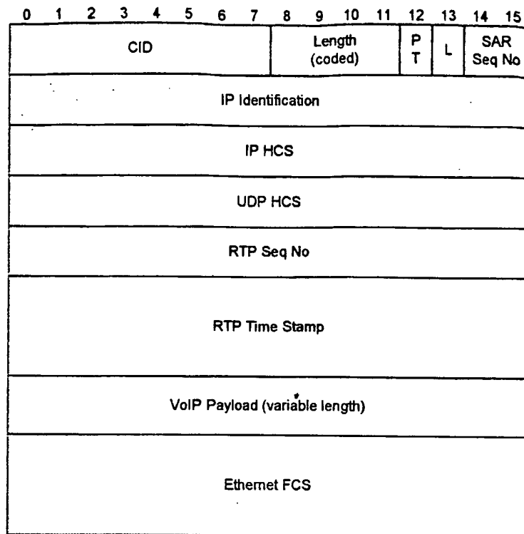
Figure 80. 20ms VoIP frame
