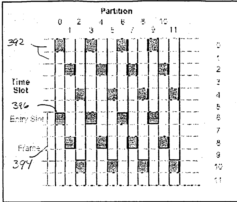
Figure 29. Partition layout for a lower-subband with a spectral spreading-factor of 4; 2x6 layout, six time-slots per frame.
