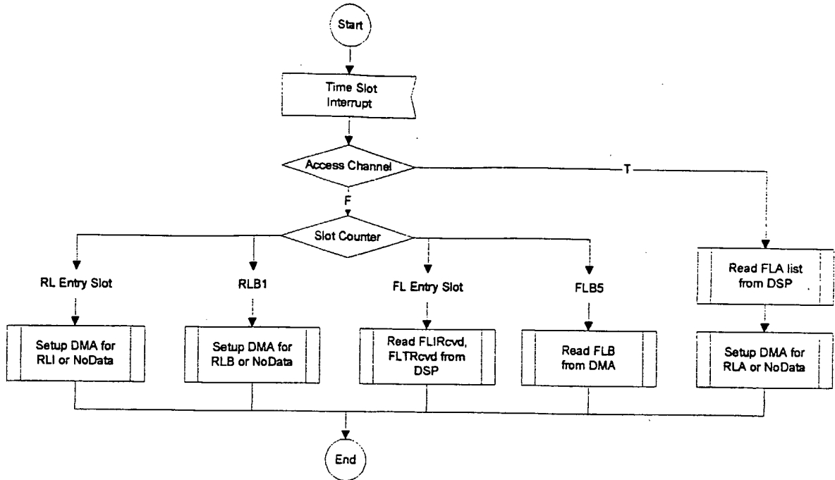
Figure 94. RU PE slot-driven component 77
