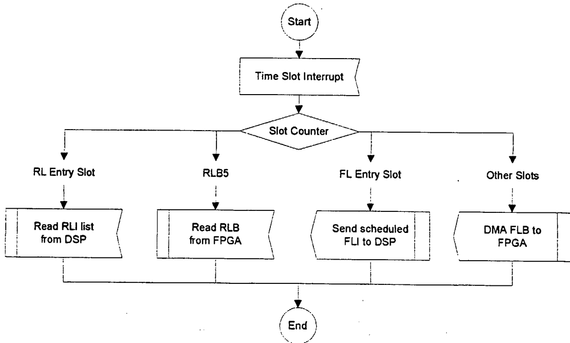
Figure 98. Base partition engine slot driven component 92
