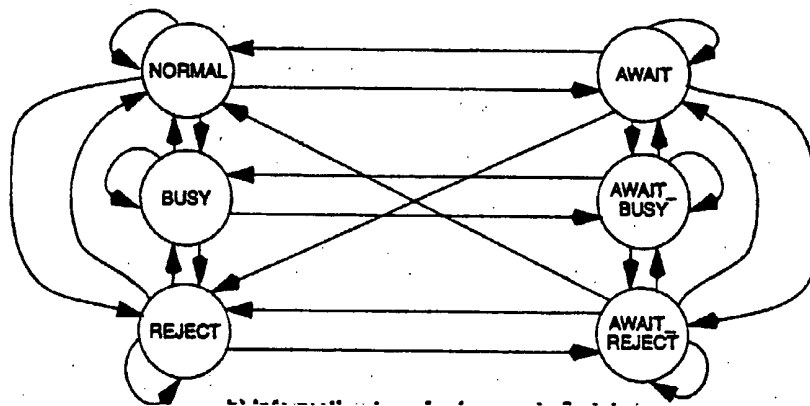
Figure 89. LLC state diagram information transfer phase
