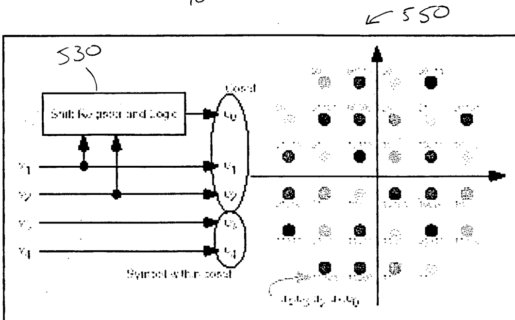
Figure 44. Generic Rate 4/5 TCM Encoder.
