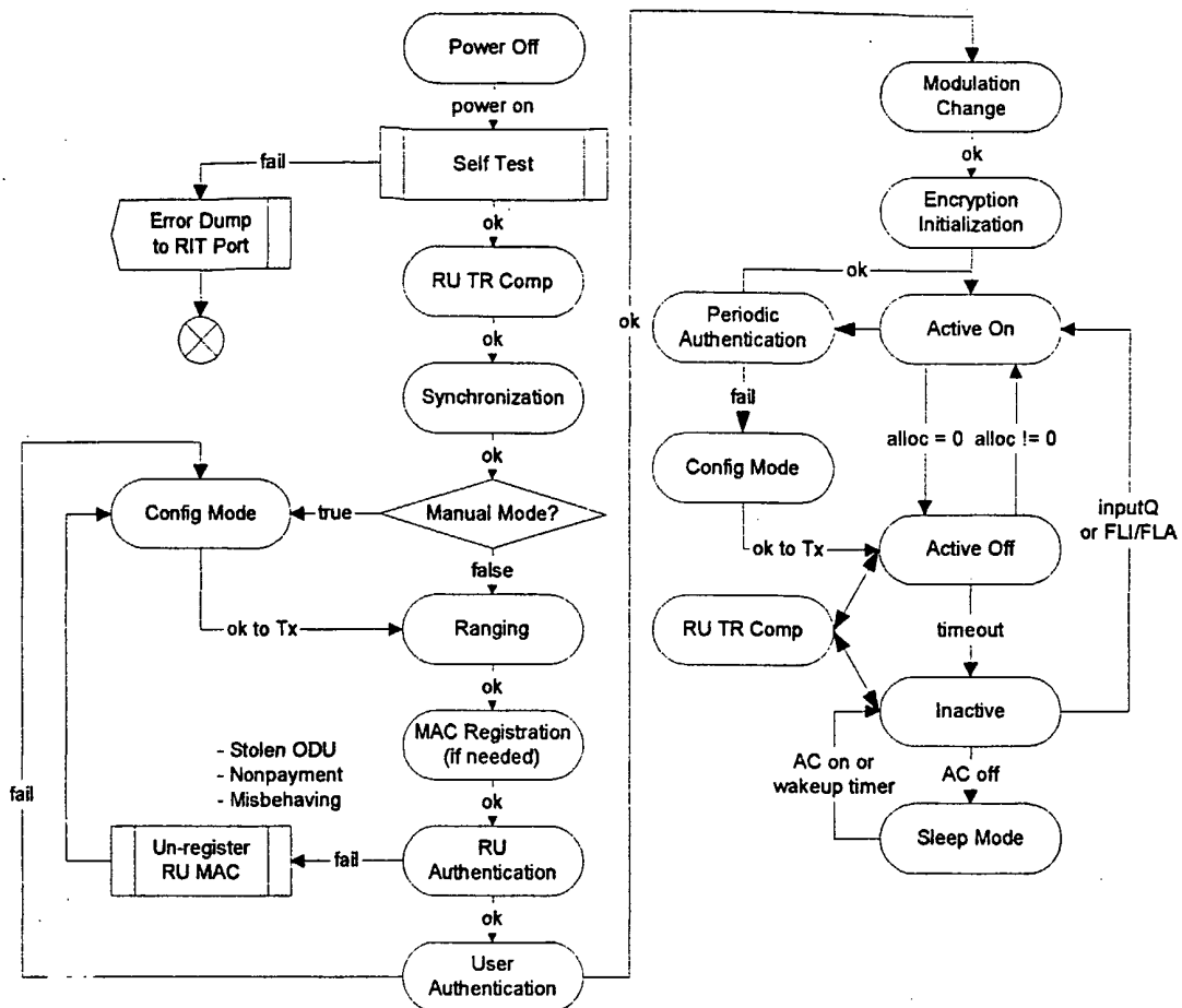
Figure 90. RU ODU state diagram.
