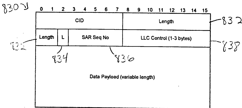
Figure 76. MAC message format 70
