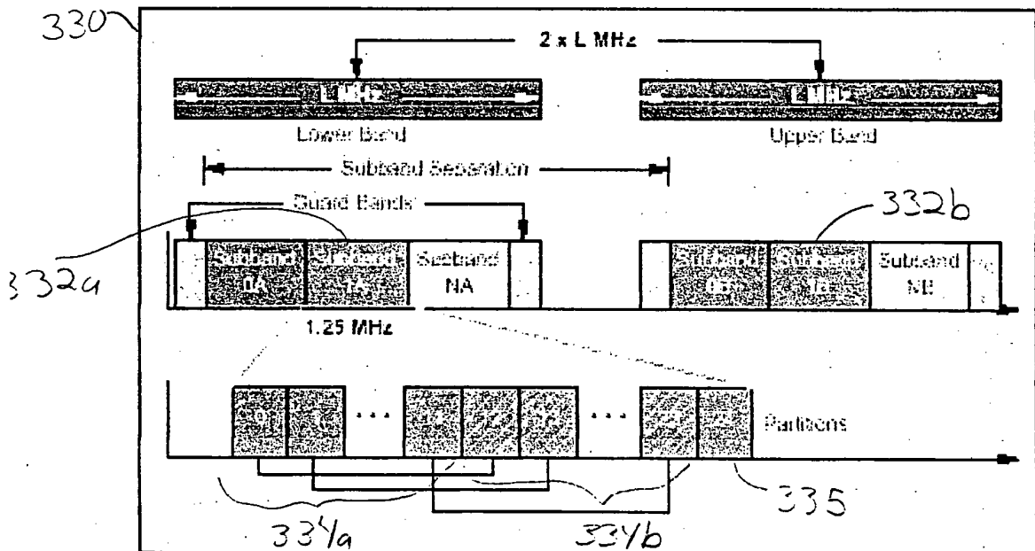
Figure 23. Frequency plan with a spreading factor of four.
