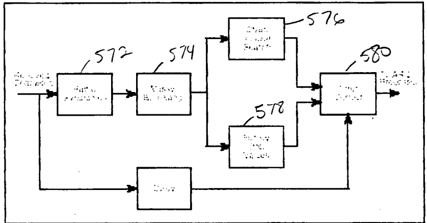
Figure 46. Generic Reed-Soloman Decoder.
