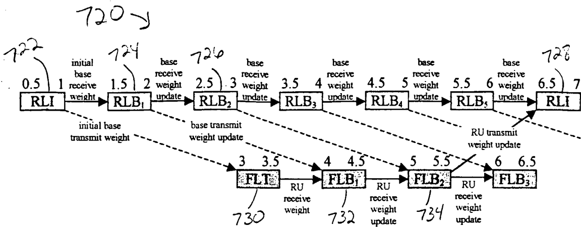
Figure 51. Weight Vector Dependencies.
