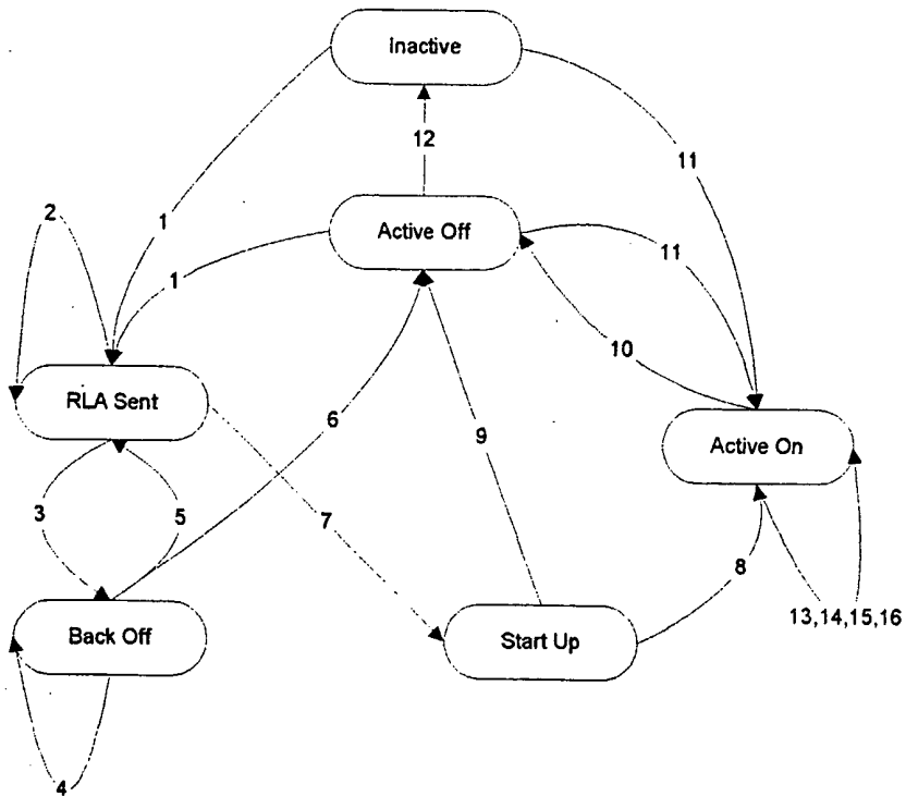
Figure 95. RU MAC scheduler state diagram. 79
