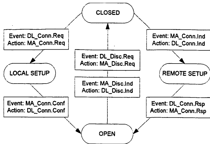
Figure 86. LLC state diagram for voice
