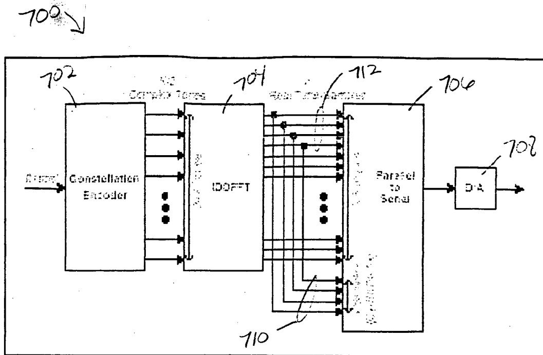
Figure 50. Functional Synthesis Block Diagram with Cyclic Prefix.
