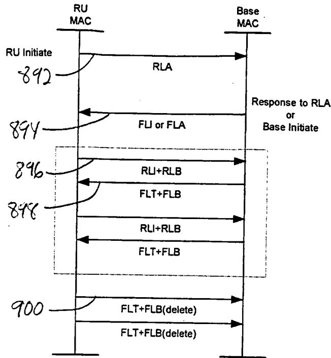
Figure 92. Connection initiation and data transfer
