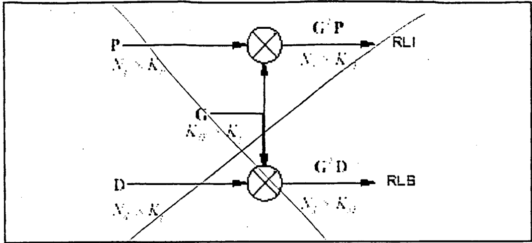
Figure 41. Forward Link Spreading Operation.
