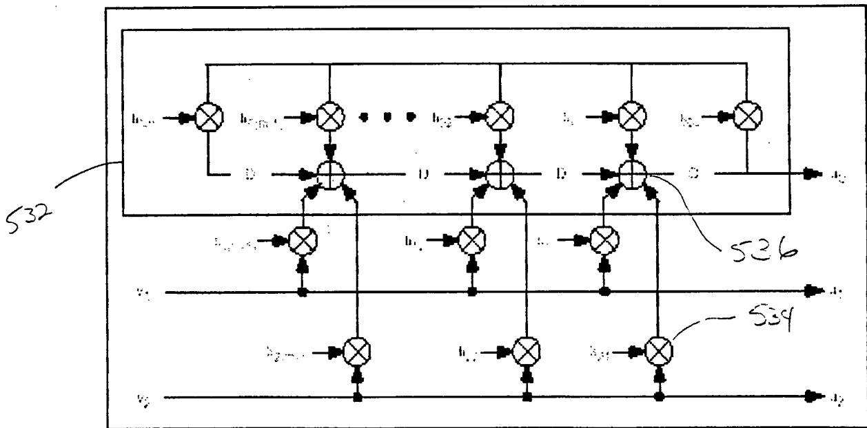
Figure 42. Rate 2/3, 2^m -state Convolutional Encoder with Feedback.
