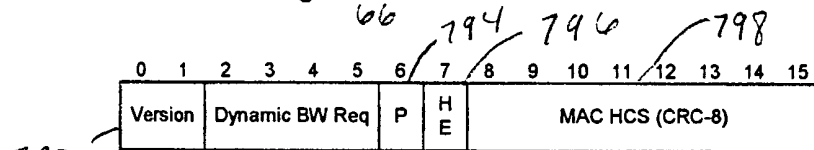
Figure 73. Reverse link common MAC header 67
