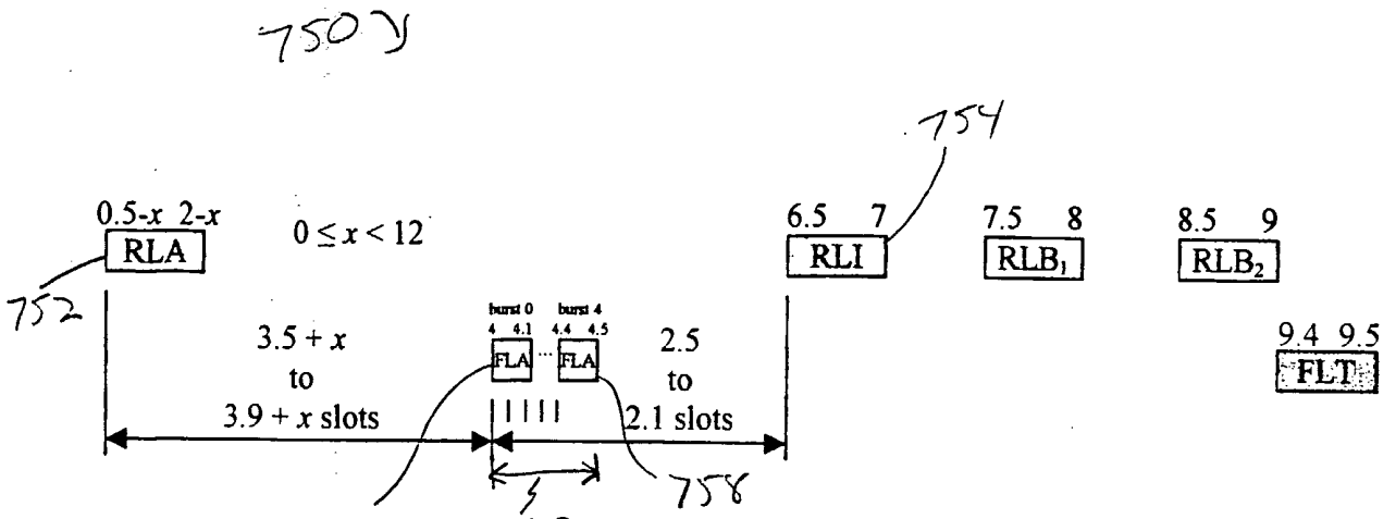
Figure 37. RLA, FLA, and RLI timing in slots. 53
