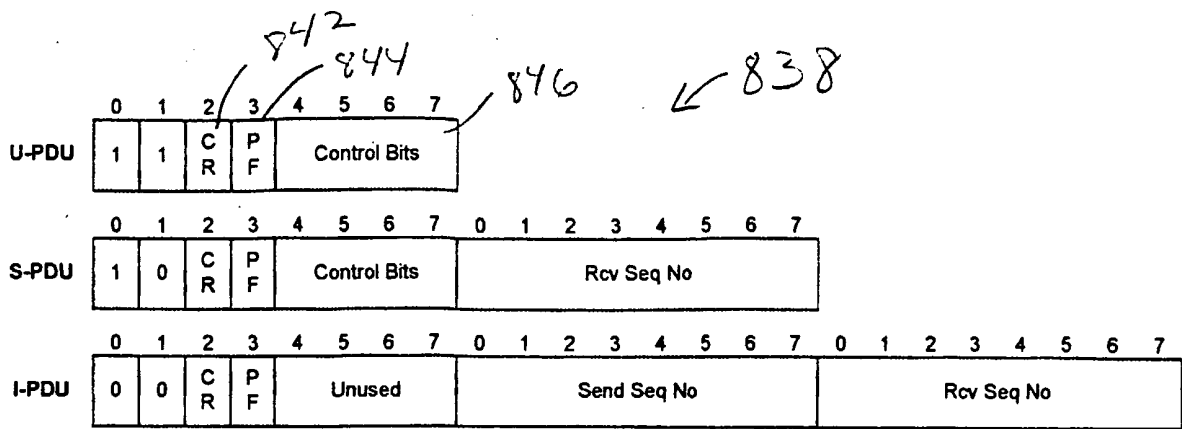
72 Figure 78. LLC control field format
