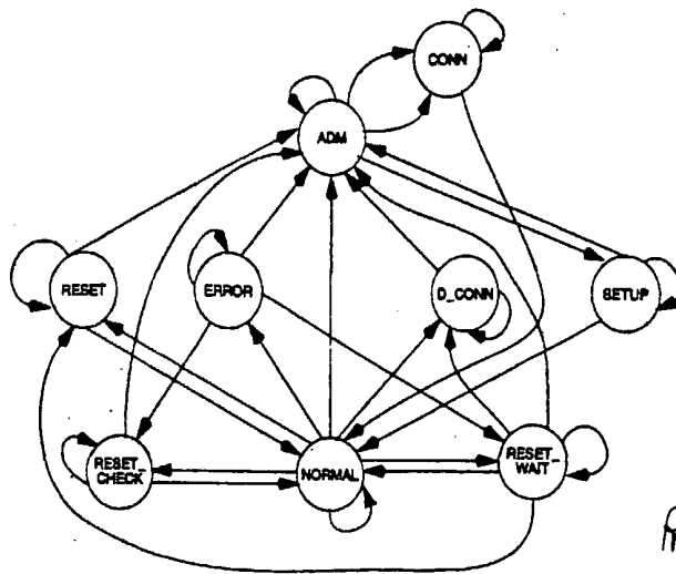
Figure 88. LLC state diagram link setup, teardown and recovery phase, prior art.
