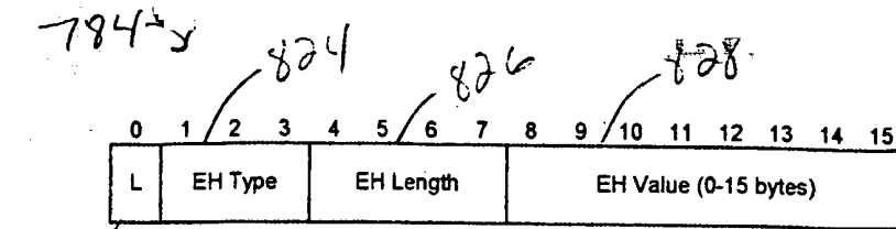
Figure 75. Extended MAC header 69
