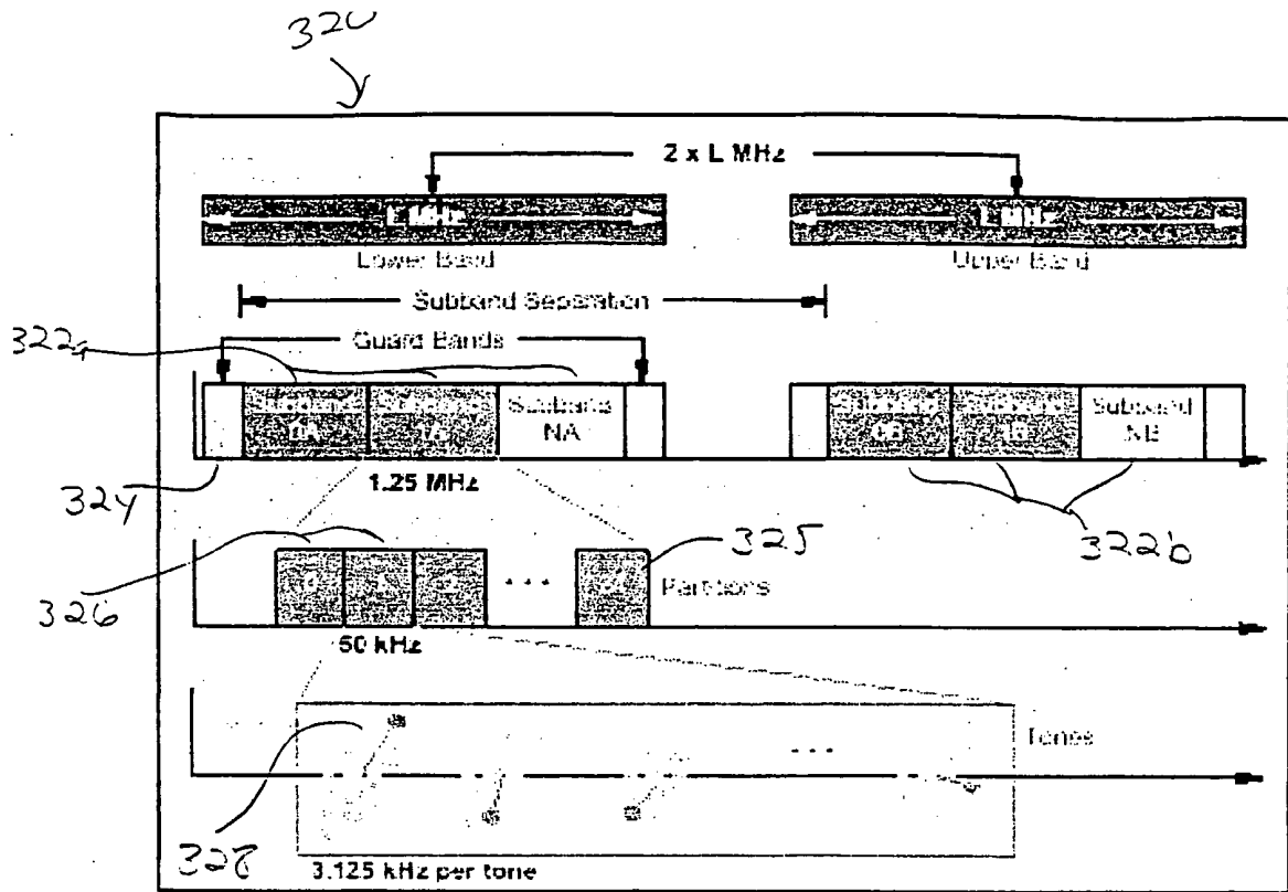
Figure 22. Frequency plan with a spectral-spreading factor of two.
