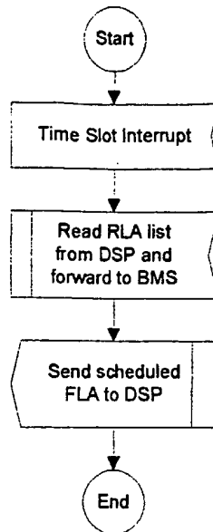
93 Figure 99. Base partition engine for the access channel.
