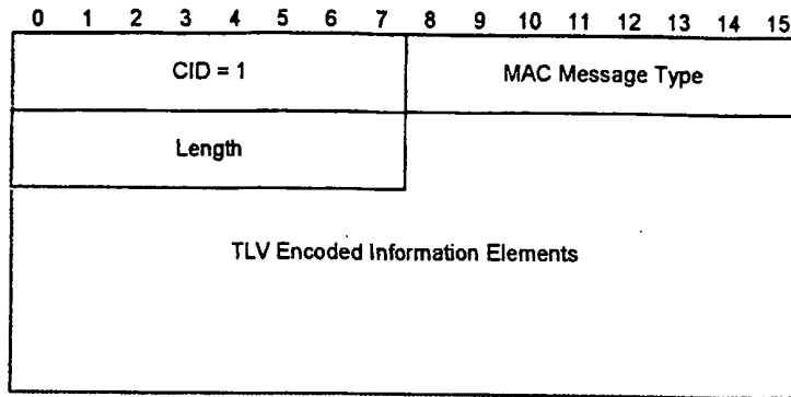
Figure 76. MAC message format 70
