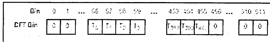
Figure 49: Mapping of Tones into IDFT-Bins.
