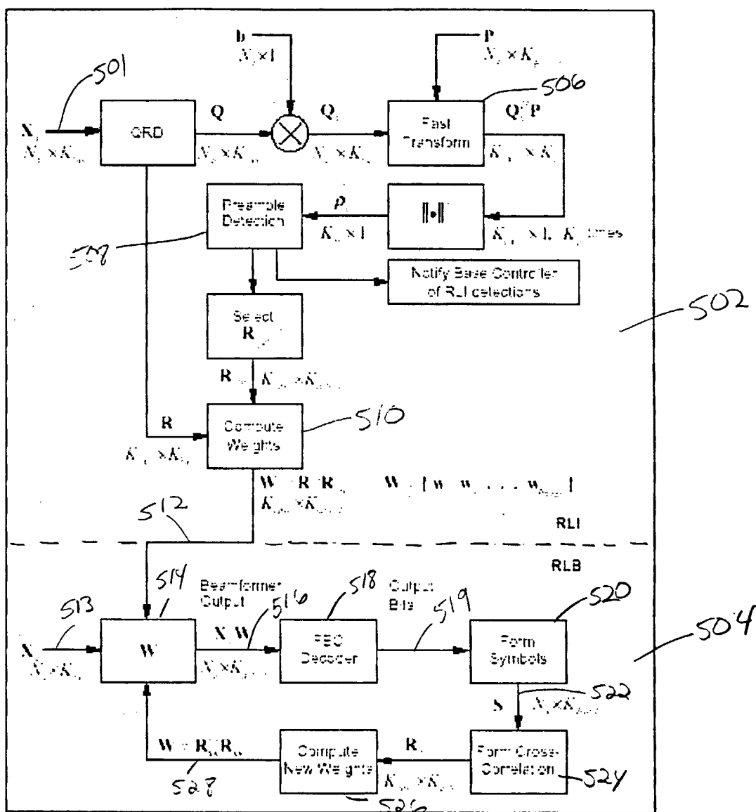
Figure 40. Base Receiver Block Diagram.
