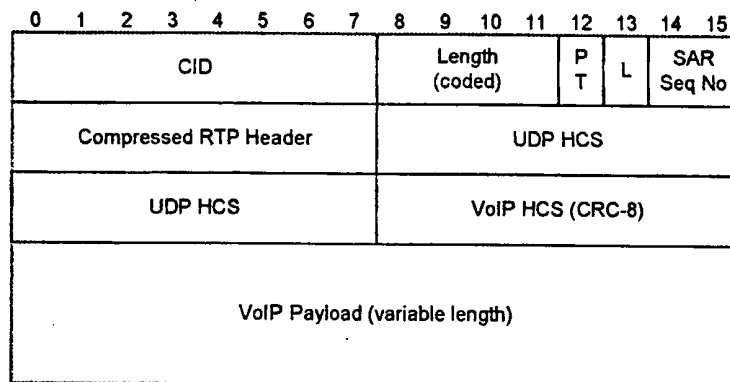
Figure 81. 10ms VoIP frame
