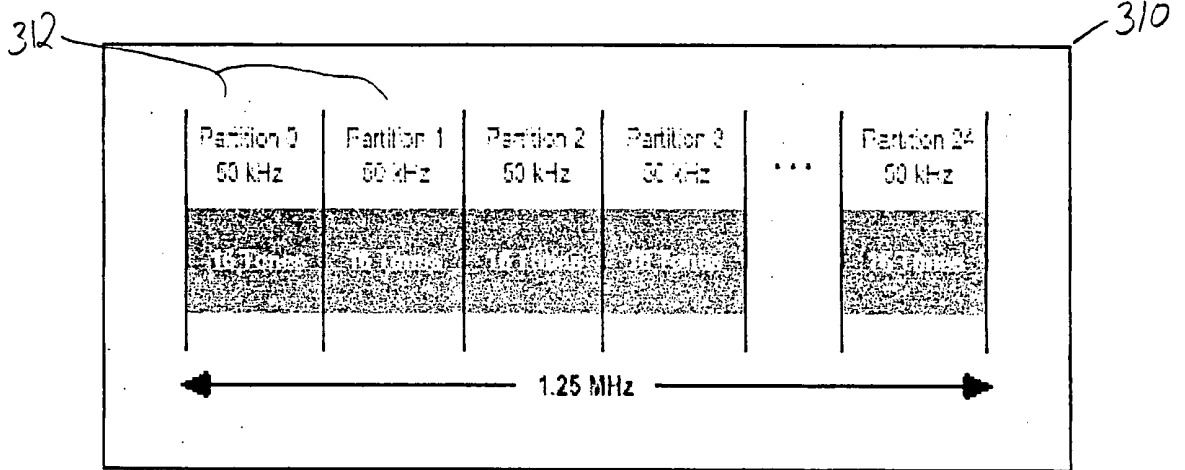
Figure 21. Tone Partitions within a Subband
