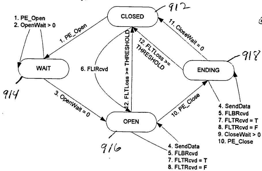
Figure 93. RU PE frame-driven component
