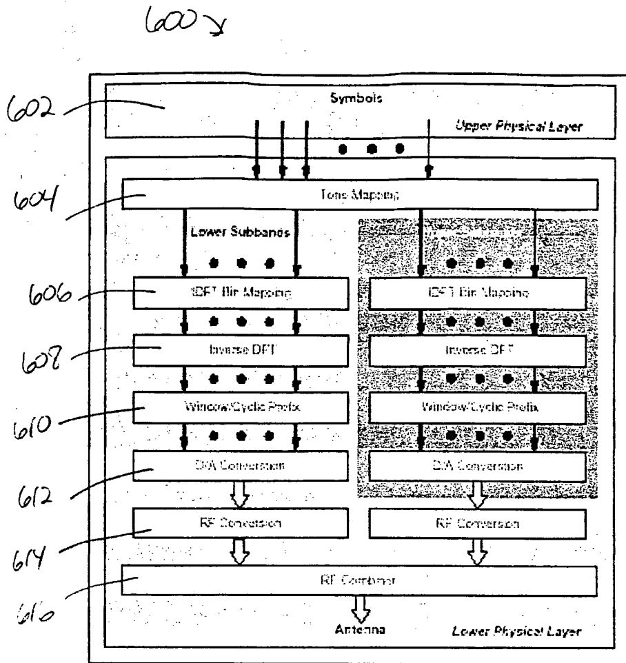
Figure 48: Physical Layer Transmission Block-Diagram.
