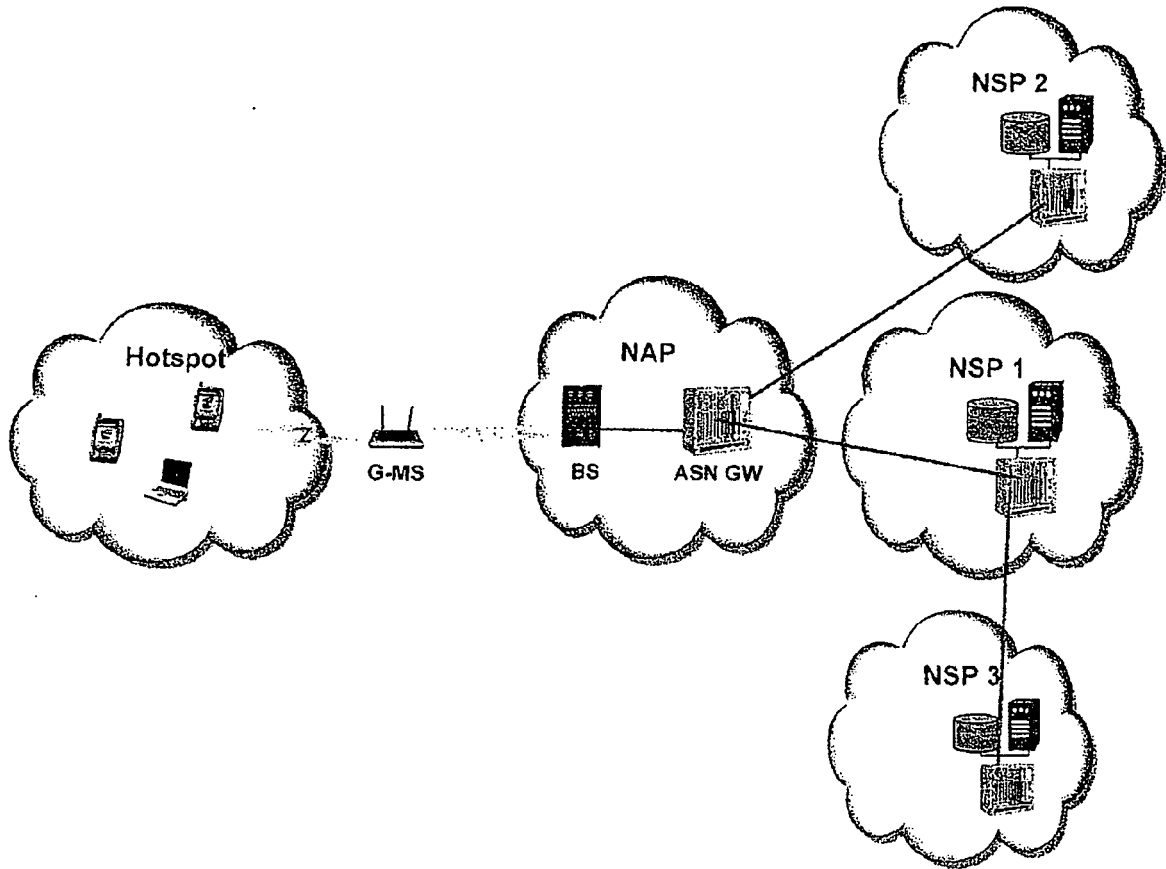
Figure 1: Architectural overview
