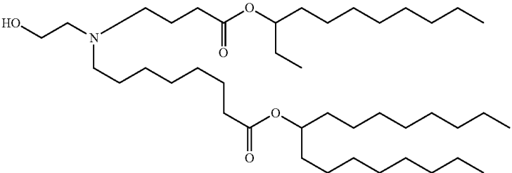
(Compound 73)
