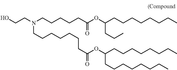
(Compound 77)
