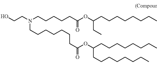
(Compound 75)
