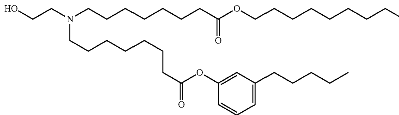
Chemical Formula: C 38 H 67 NO 5 Molecular Weight: 617.96
