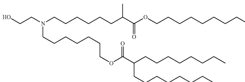
Chemical Formula: C 45 H 89 NO 5 Molecular Weight: 724.209
