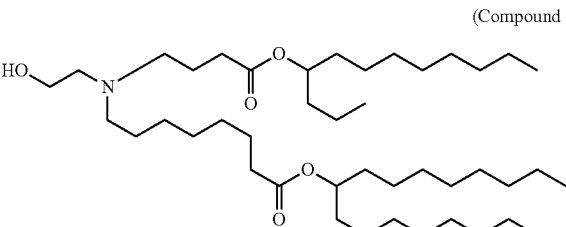
(Compound 76)
