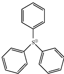
Structure of Sulfonium Salt Compound TN-2
