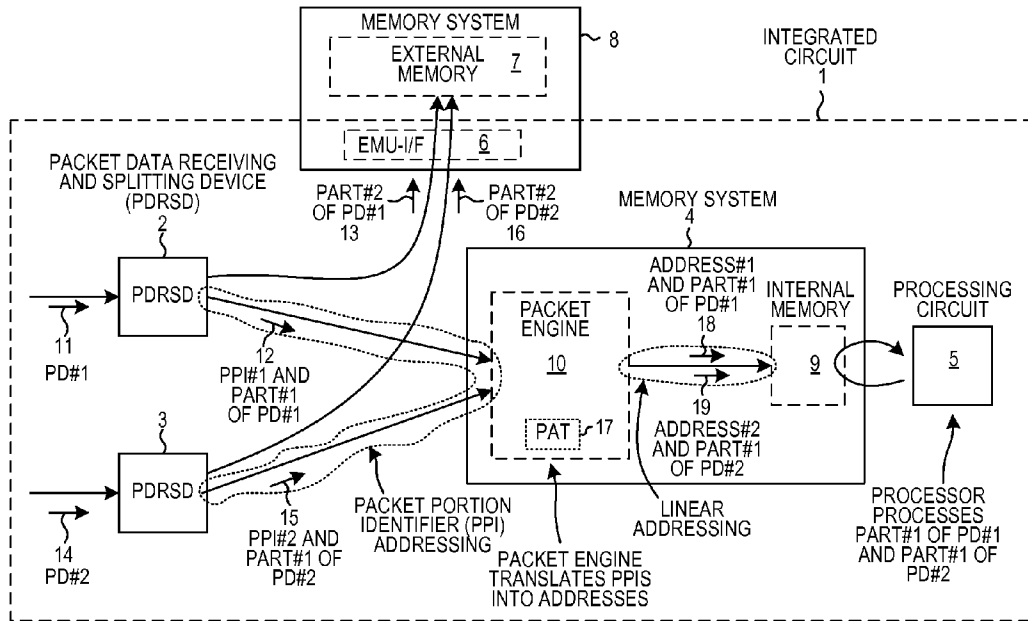
MEMORY SYSTEM WITH PPI ADDRESSING
