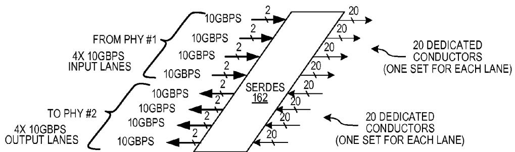
ONE SERDES CIRCUIT
