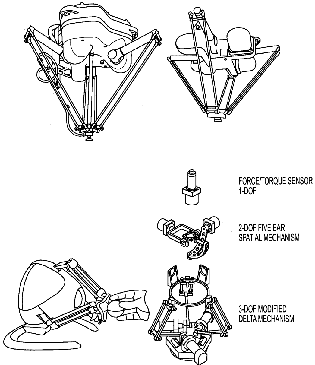
FIG. 7 (PRIOR ART)
