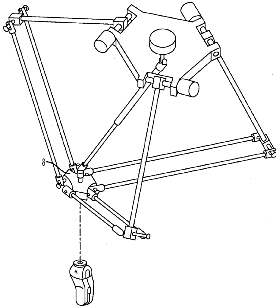
FIG. 6 (PRIOR ART)
