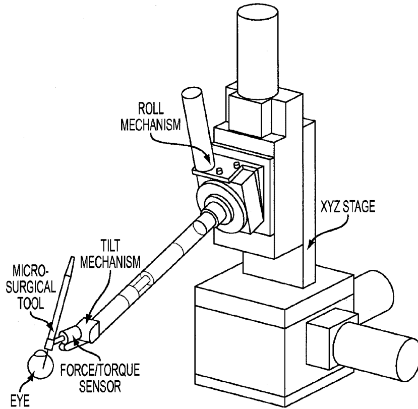
FIG. 5 (PRIOR ART)
