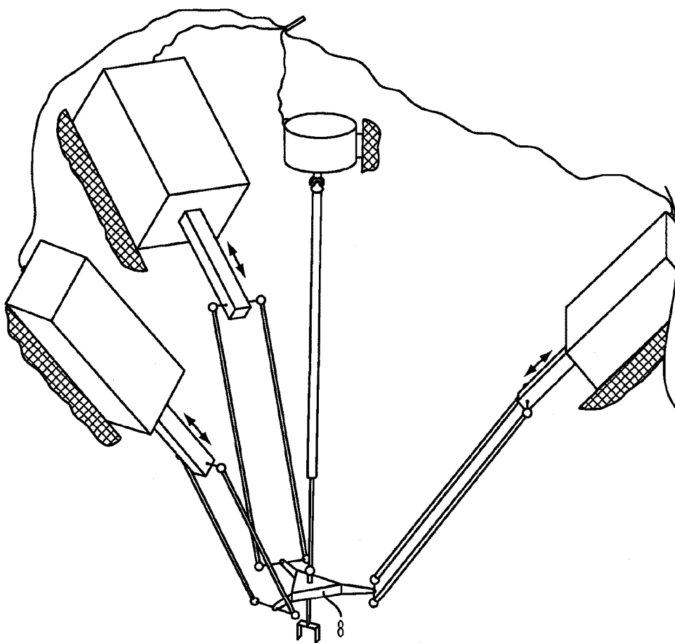
FIG. 10 (PRIOR ART)
