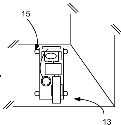
Closeup Diagram of Frame with Leveling Apparatus Attached Fig. 1D
