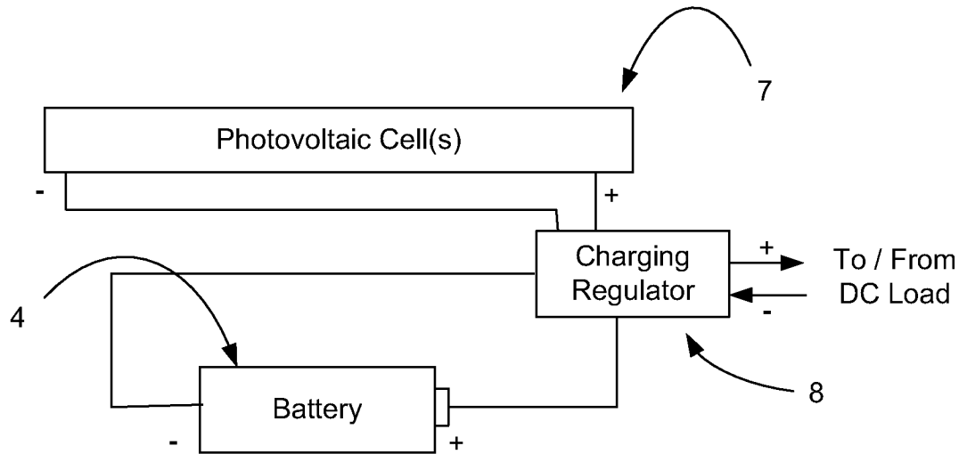
Solar Charger Diagram Fig. 4A
