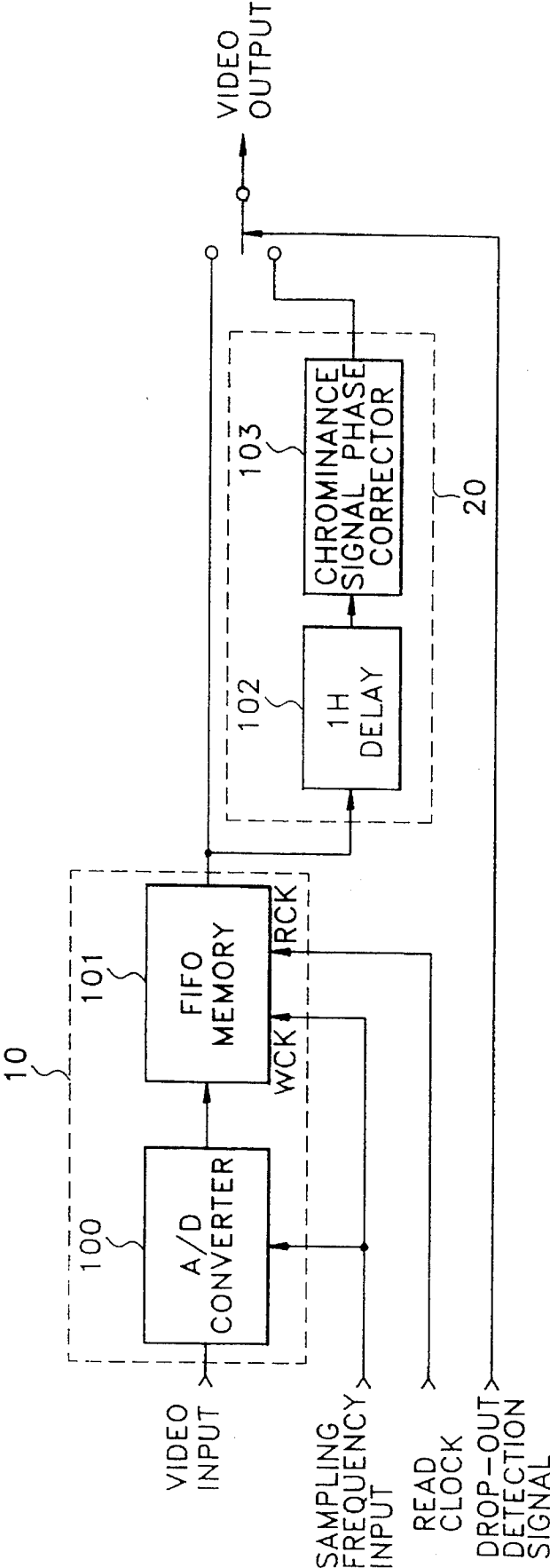
FIG. 1 (PRIOR ART)
