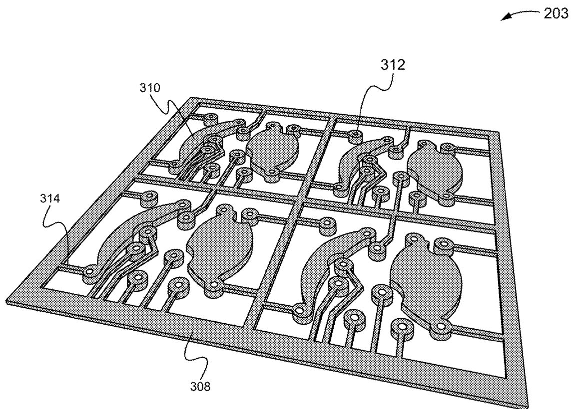
Top View 2nd Leadframe
