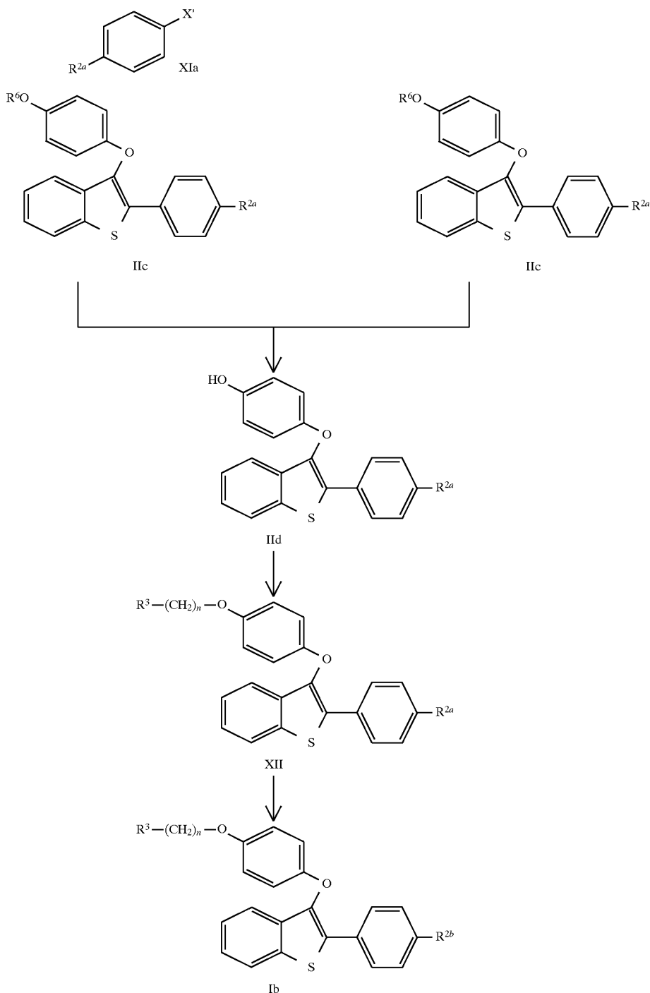
-continued Scheme IV
