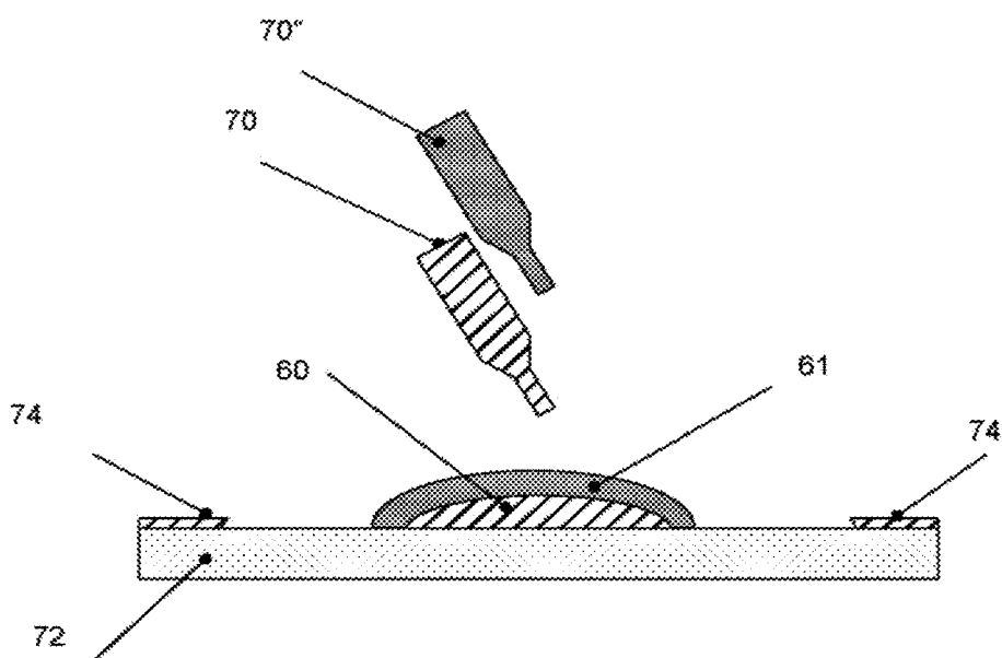
FIG. 33A - Dispensing of 2 adhesive beads
