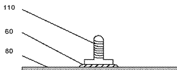
FIG. 43A. An adhesively bonded metallic fasteners to a composite panel
