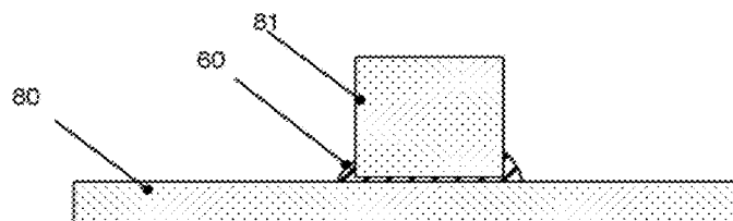
FIG. 31A - Adhesive dispense on composite substrate
