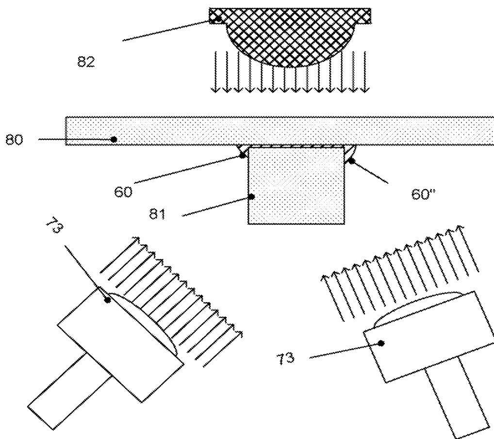
FIG. 32. Additional UV energy added to cure fillets
