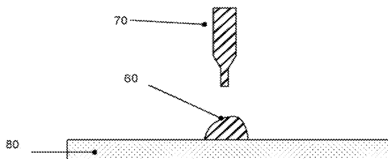
FIG. 31A - Adhesive dispense on composite substrate
