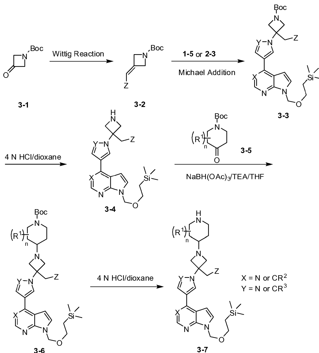
Scheme 3
