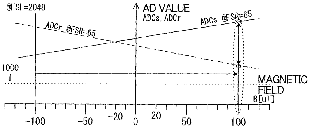
SPAN ADJUSTMENT (SC08)
