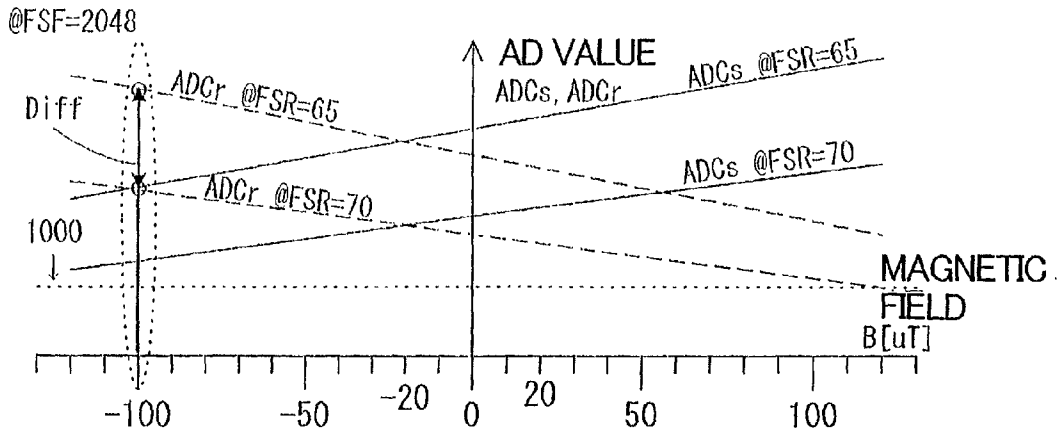
SPAN ADJUSTMENT (SC07)
