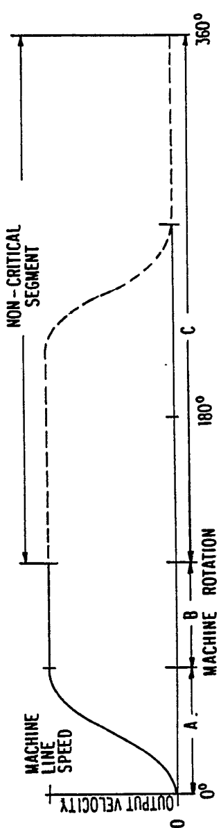
FIG. 3 SINGLE FEED
