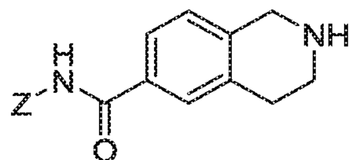
Formula LX
