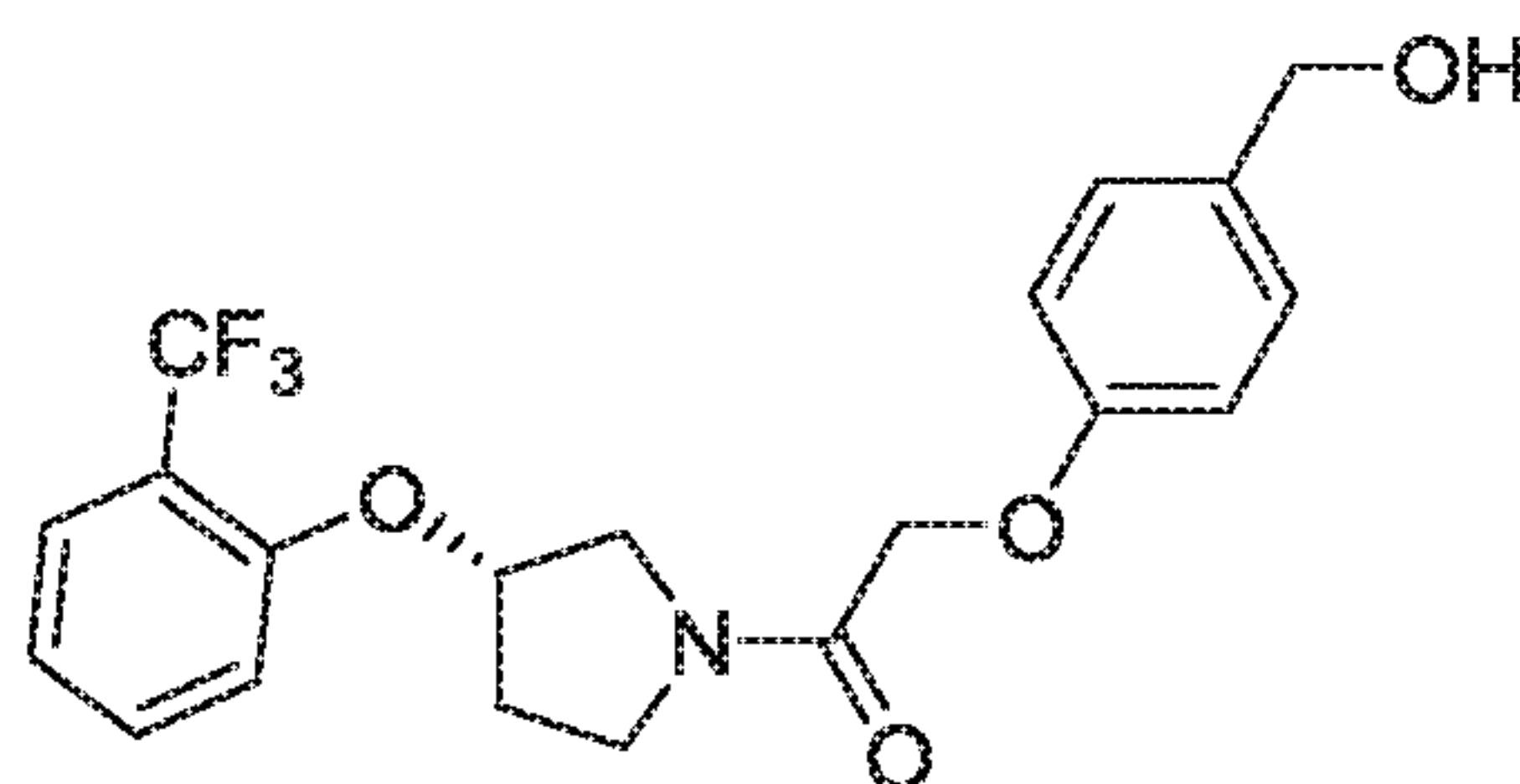
Formula LXI
