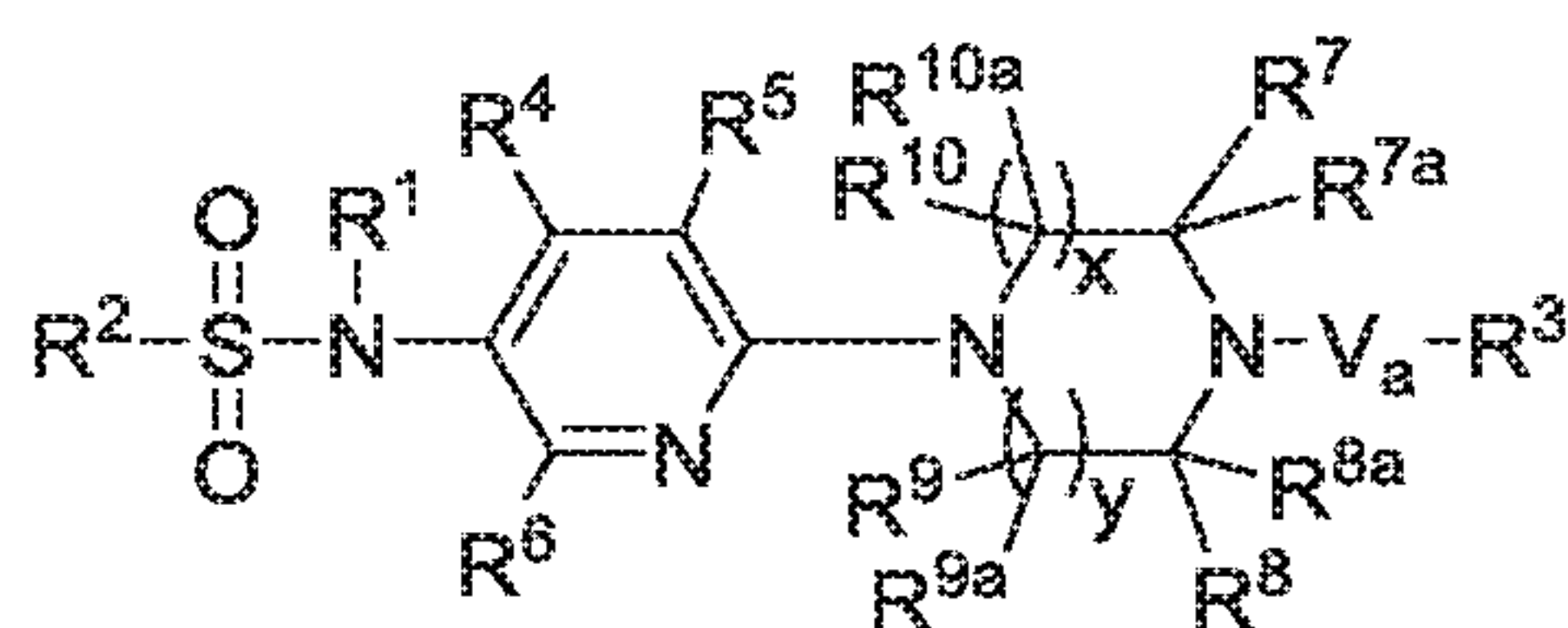
(IVd)
