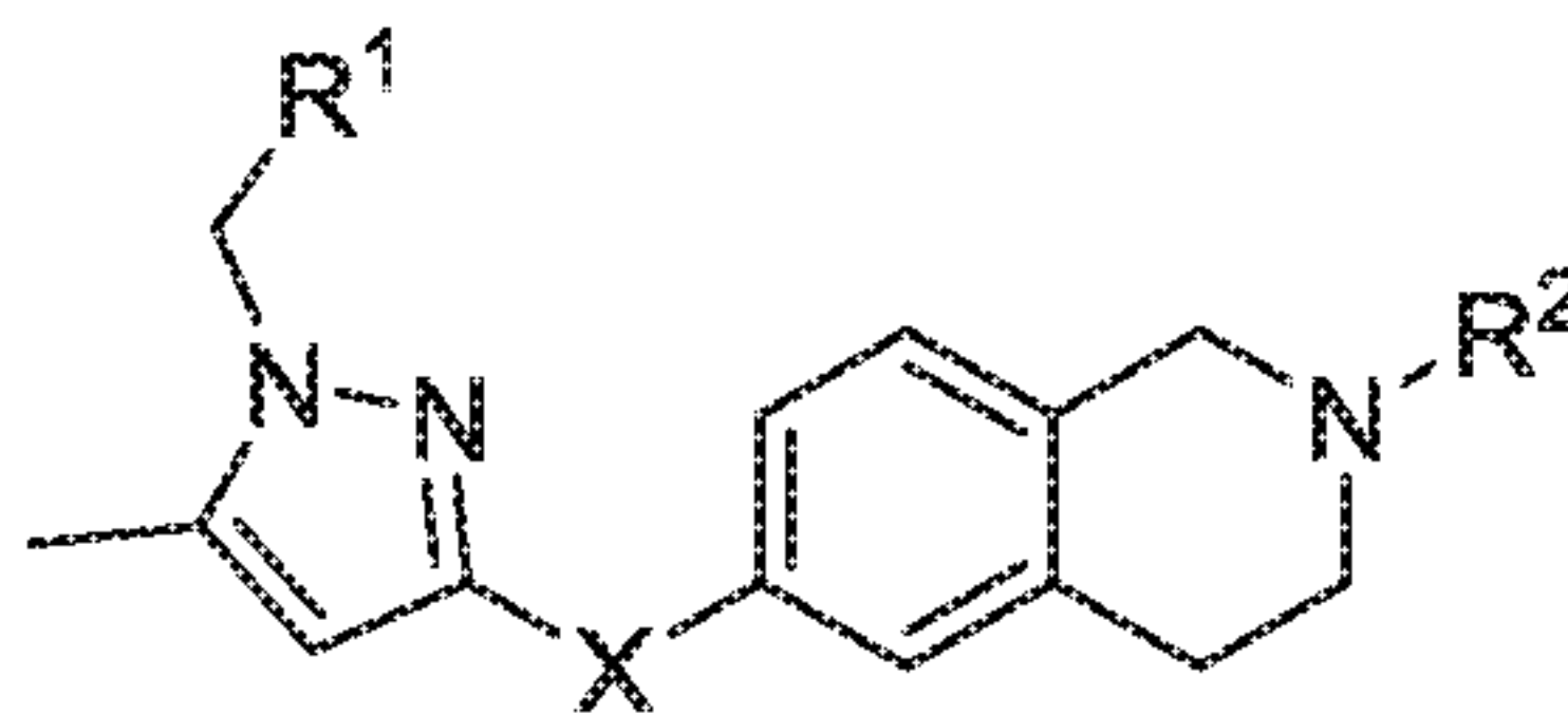
Formula LVII
