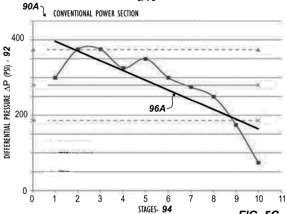
FIG. 5C (PRIOR ART)
