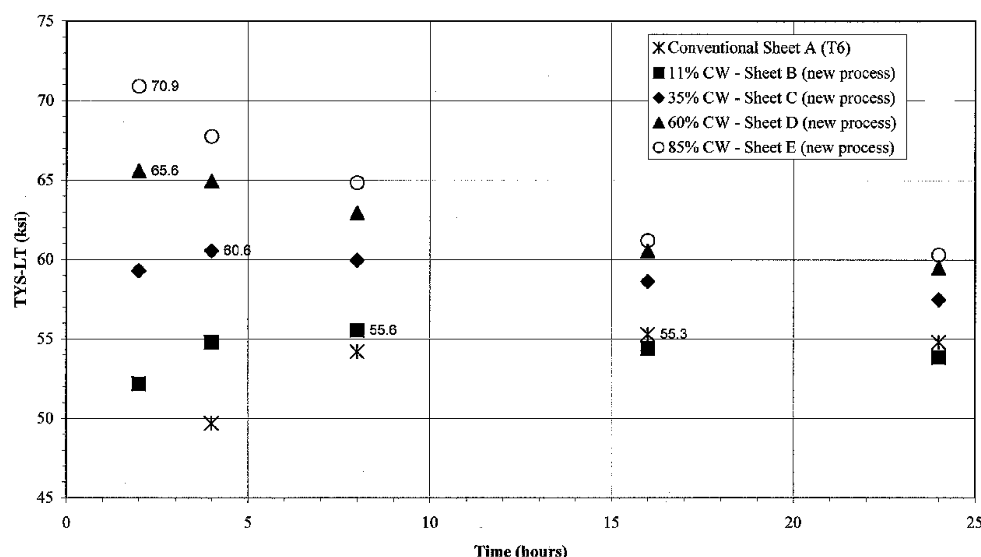
FIG. 16 - TYS v. Time at 350F
