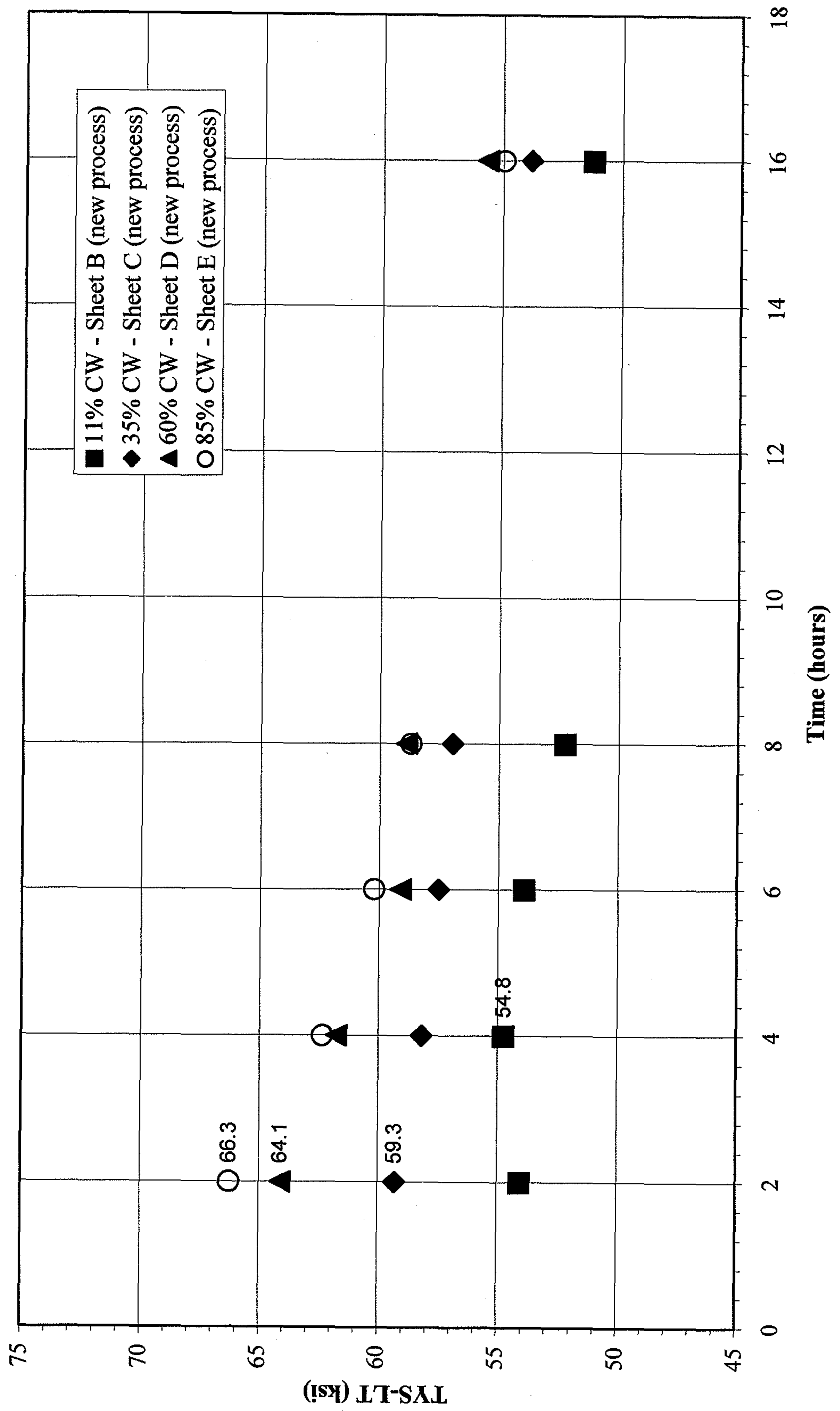
FIG. 17 - TYS v. Time at 375F
