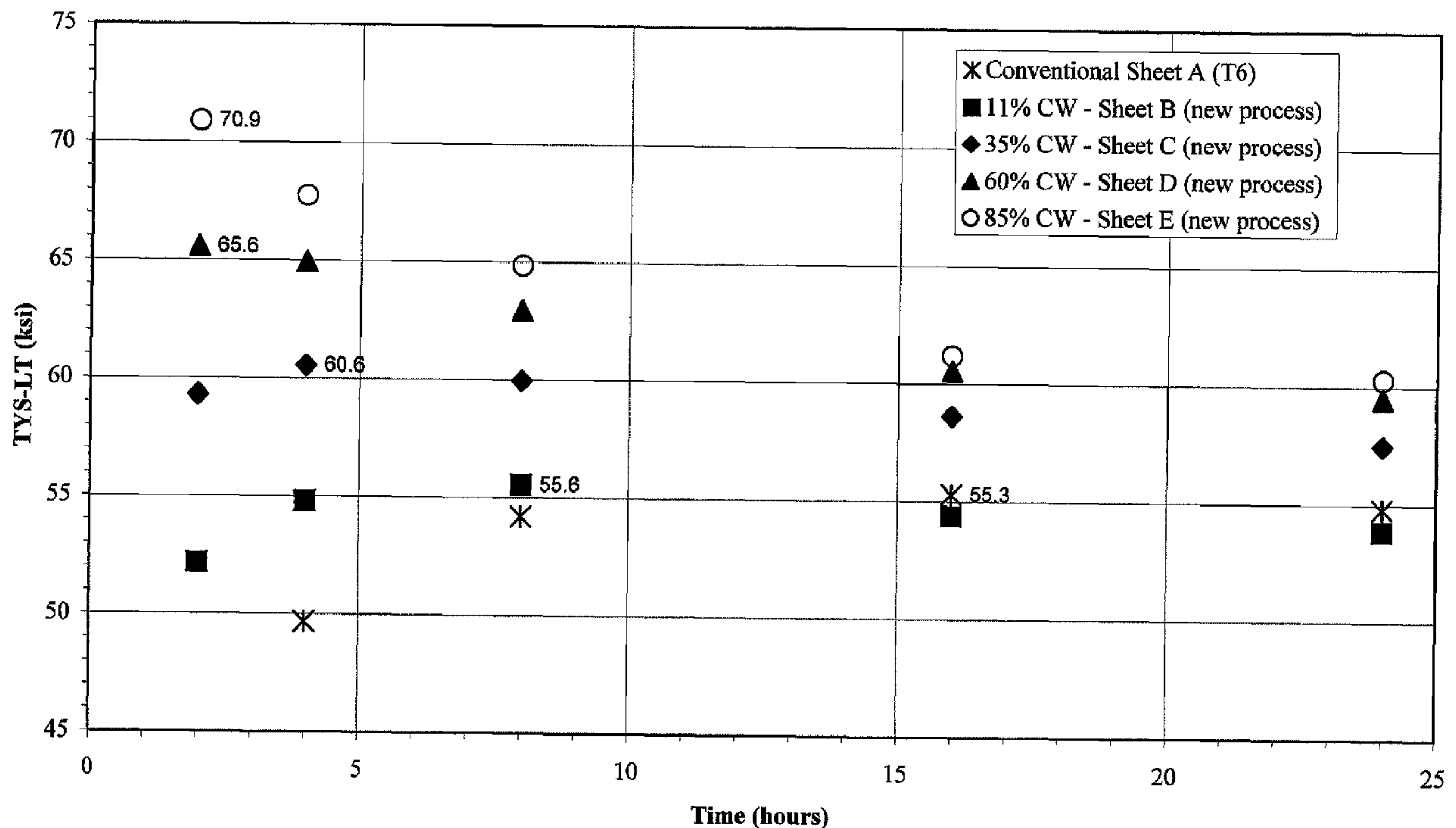
FIG. 16 - TYS v. Time at 350F
