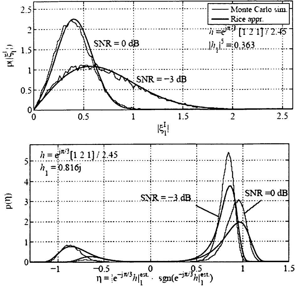
Fig. 19. Estimation of a complex channel impulse response ( h = e^{j\pi/3}[1, 2, 1]/\sqrt{6} ): Numerical evaluation of the amplitude distribution of the 5 th moment of the strongest tap (top) and the projected tap distribution \hat{h}_1 derived from it (bottom).
