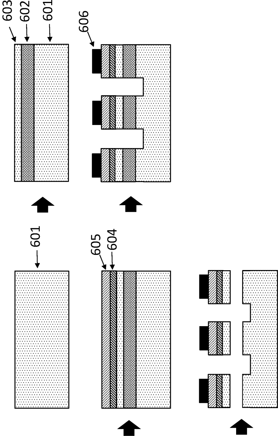
Figure 6: engineered substrate using included sacrificial layers
