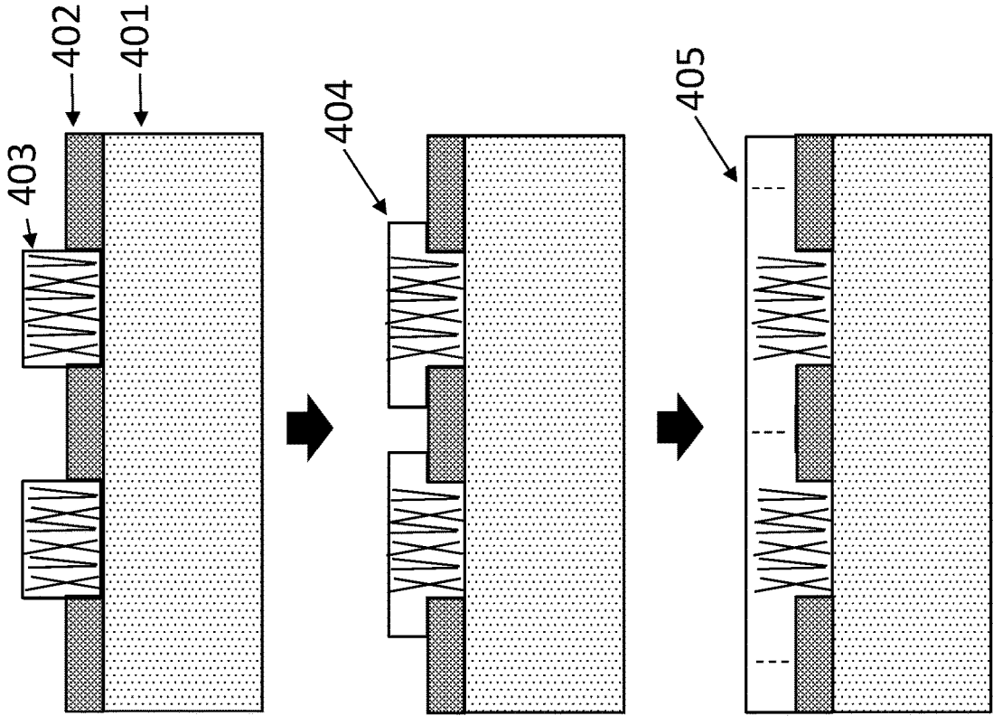
Figure 4: engineered substrate using lateral overgrowth
