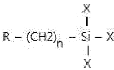
Chemical Formula 2
