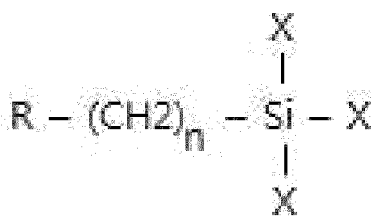
Chemical Formula 2
