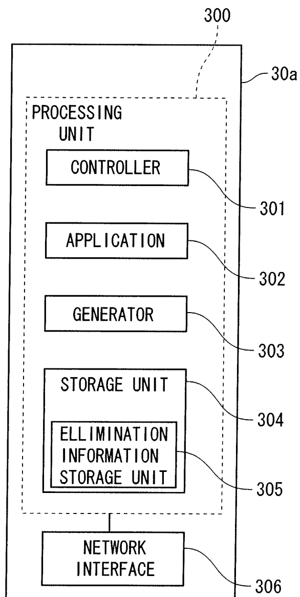
DIAGRAM SHOWING AN EXAMPLE OF STRUCTURE OF HOST COMPUTER OF SECOND EMBODIMENT
