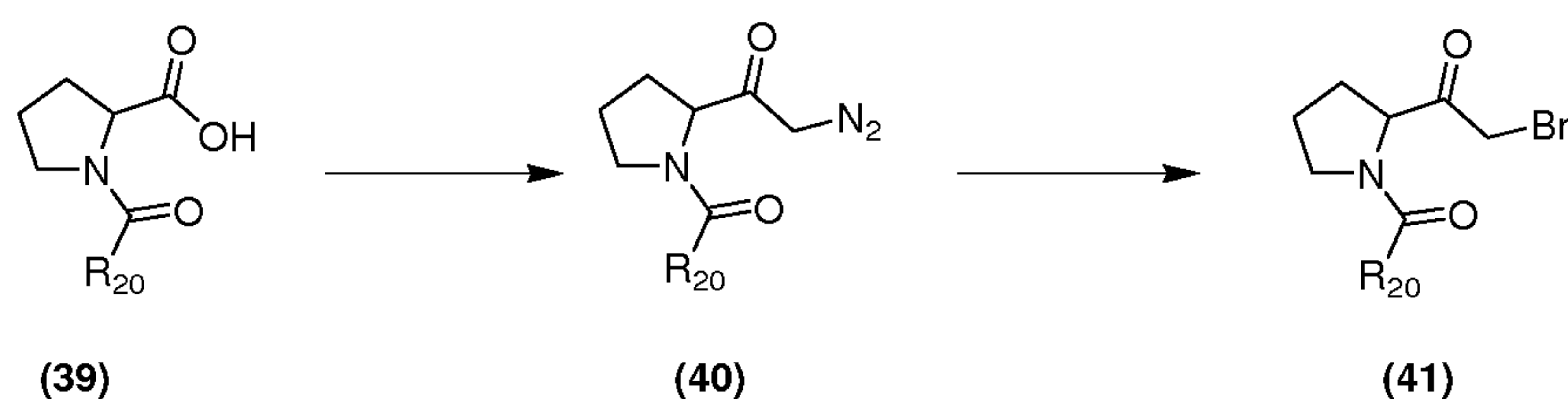
Scheme XVIII
