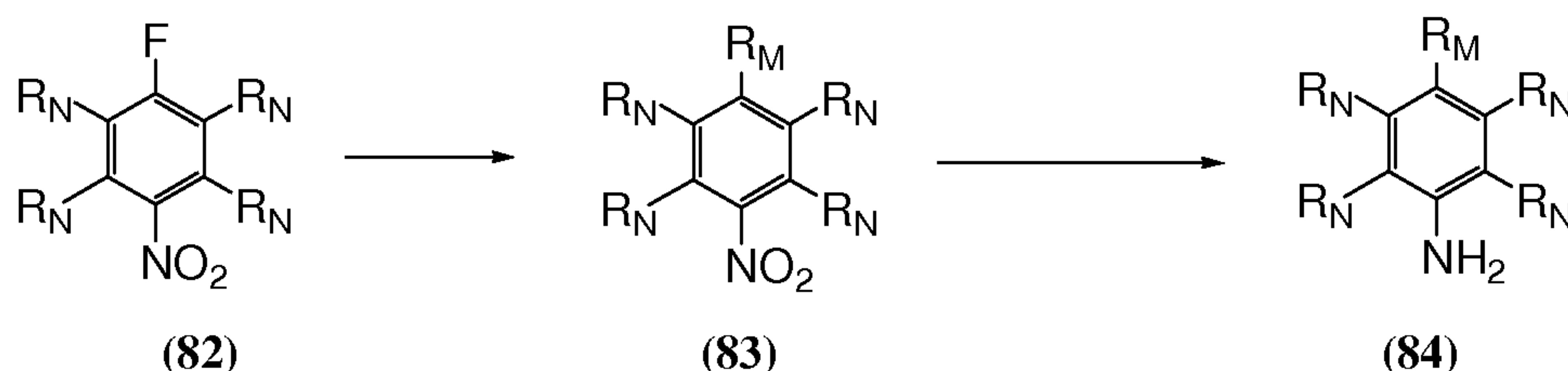
Scheme XXV
