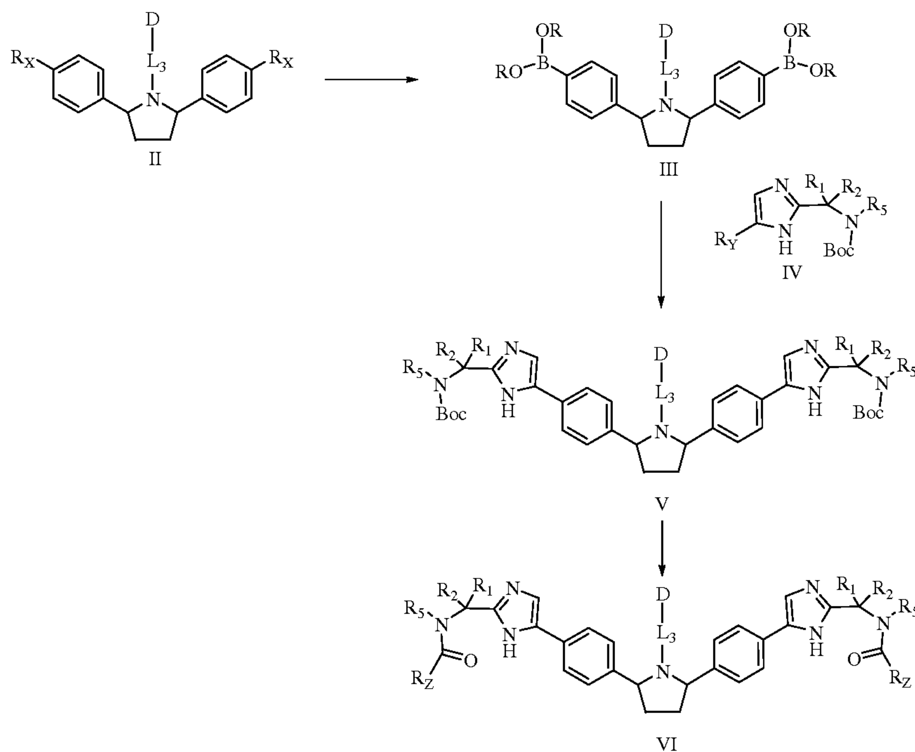
Scheme VII
