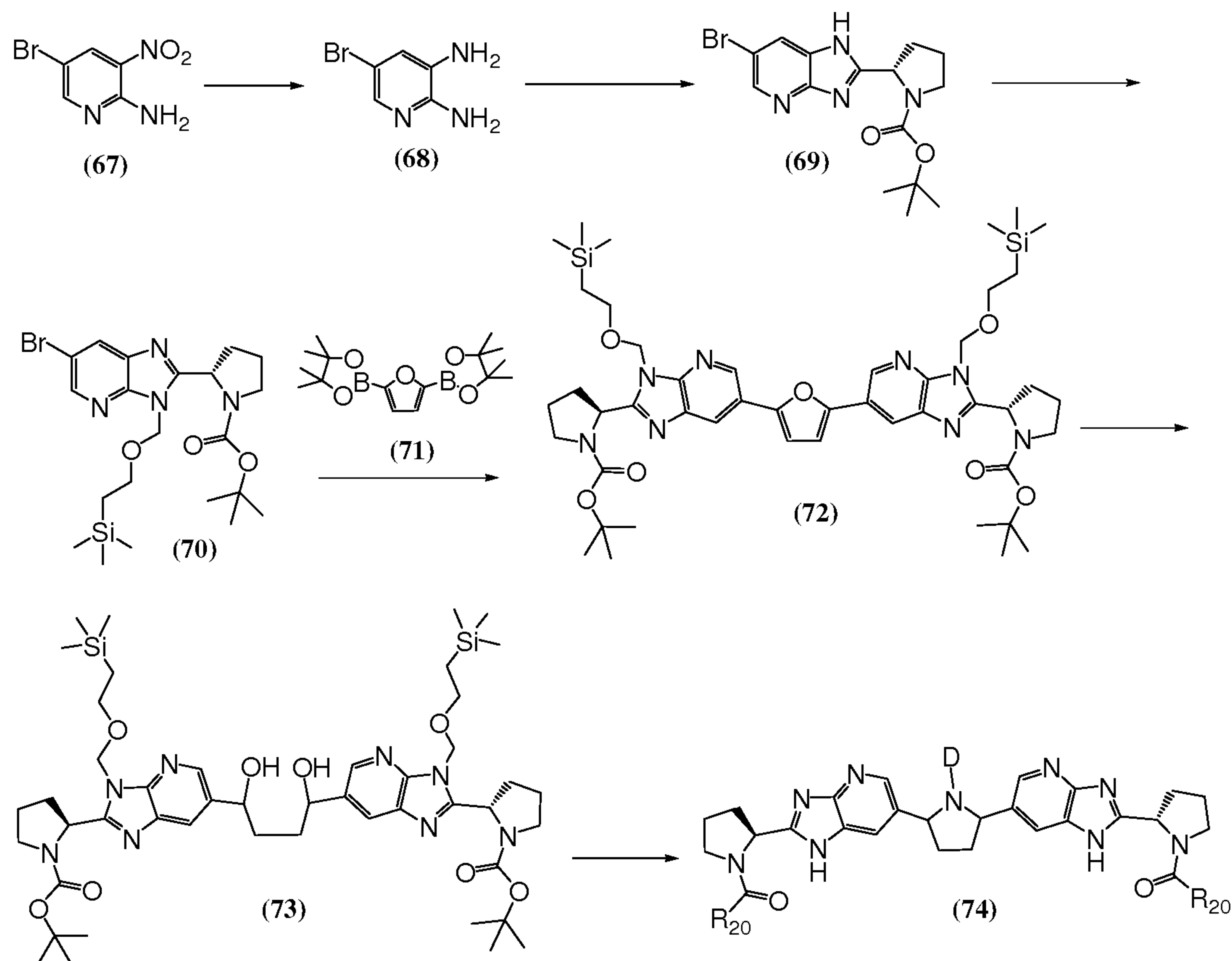
Scheme XXIII
