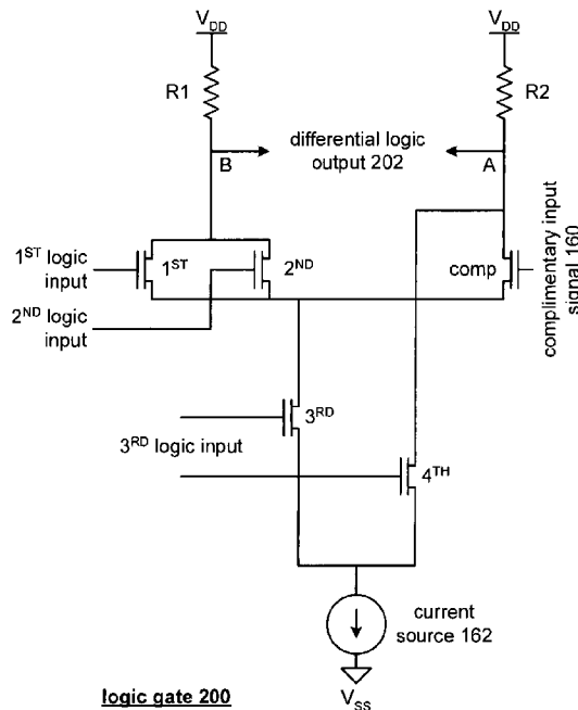
logic gate 200
