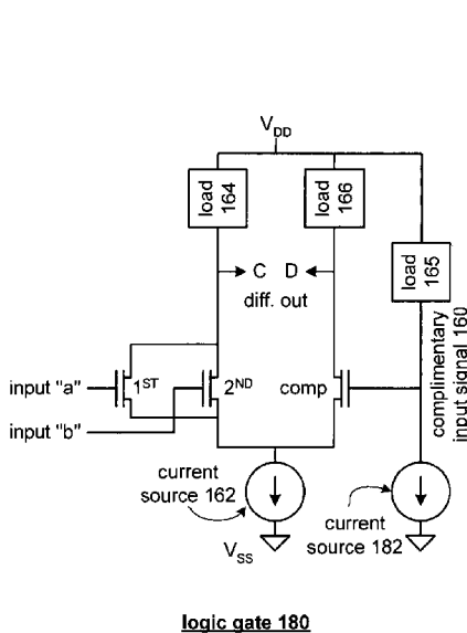
logic gate 180
