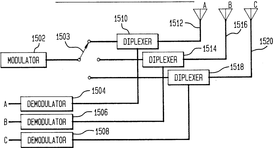
TRANSFER STATION ANTENNA IMPLEMENTATION
