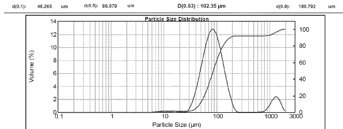
Fig. 3: Particle size analysis of the primary particles treated with the polymer and sheared before measuring.
