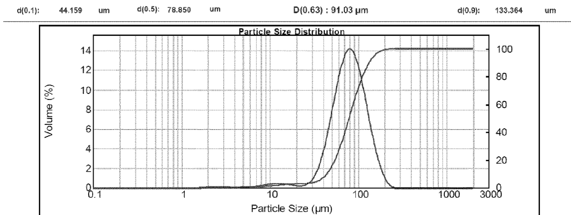
Fig. 2: Particle size analysis of the primary particles.
