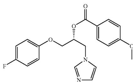
4-methoxy-benzoic acid 1-imidazol-1-yl methyl-2-(4-fluorophenoxy)-ethyl ester;
