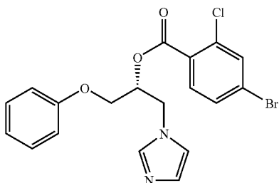
4-bromo-2-chloro-benzoic acid 1-imidazol-1-yl methyl-2-phenoxymethyl ester;
