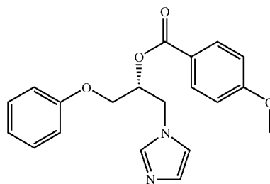
(R) 4-methoxy-benzoic acid 1-imidazol-1-yl methyl-2-phenoxy-ethyl ester;
