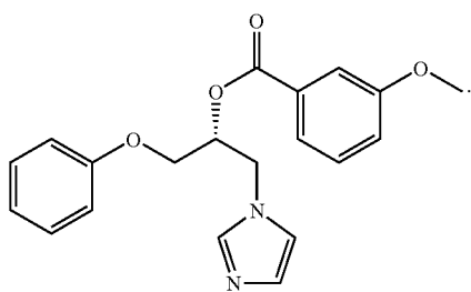
3-methoxy-benzoic acid 1-imidazol-1-yl methyl-2-phenoxy-ethyl ester;
