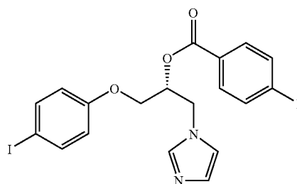
4-iodo-benzoic acid 1-imidazol-1-yl methyl-2-(4-iodophenoxy)-ethyl ester;
