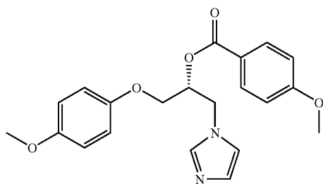
4-methoxy-benzoic acid 1-imidazol-1-yl methyl-2-(4-methoxyphenoxy)-ethyl ester;
