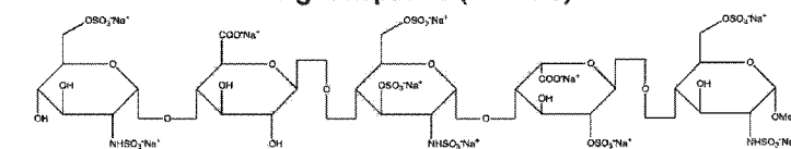
General structure of Unfractionated Heparin (UFH) and Low Molecular Weight heparins (LMWHs)
