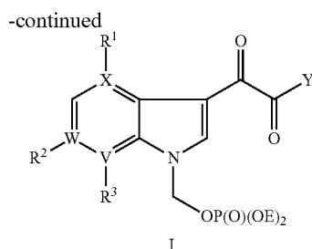
Compounds of Claim 1 E = hydrogen, or as defined to form pharmaceutically acceptable mono or bis salt
