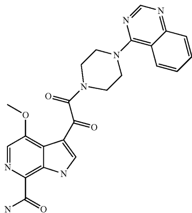
4-methoxy-3-(2-oxo-2-(4-(quinazolin-4-yl)piperazin-1-yl)acetyl)-1H-pyrrolo[2,3-c]pyridine-7-carboxamide
