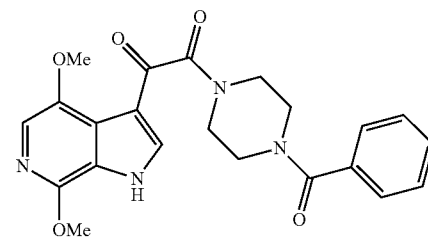
IVa Mol. Wt. = 422.43
