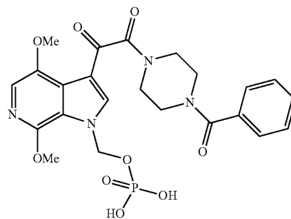
Iac Mol. Wt. = 532.44
