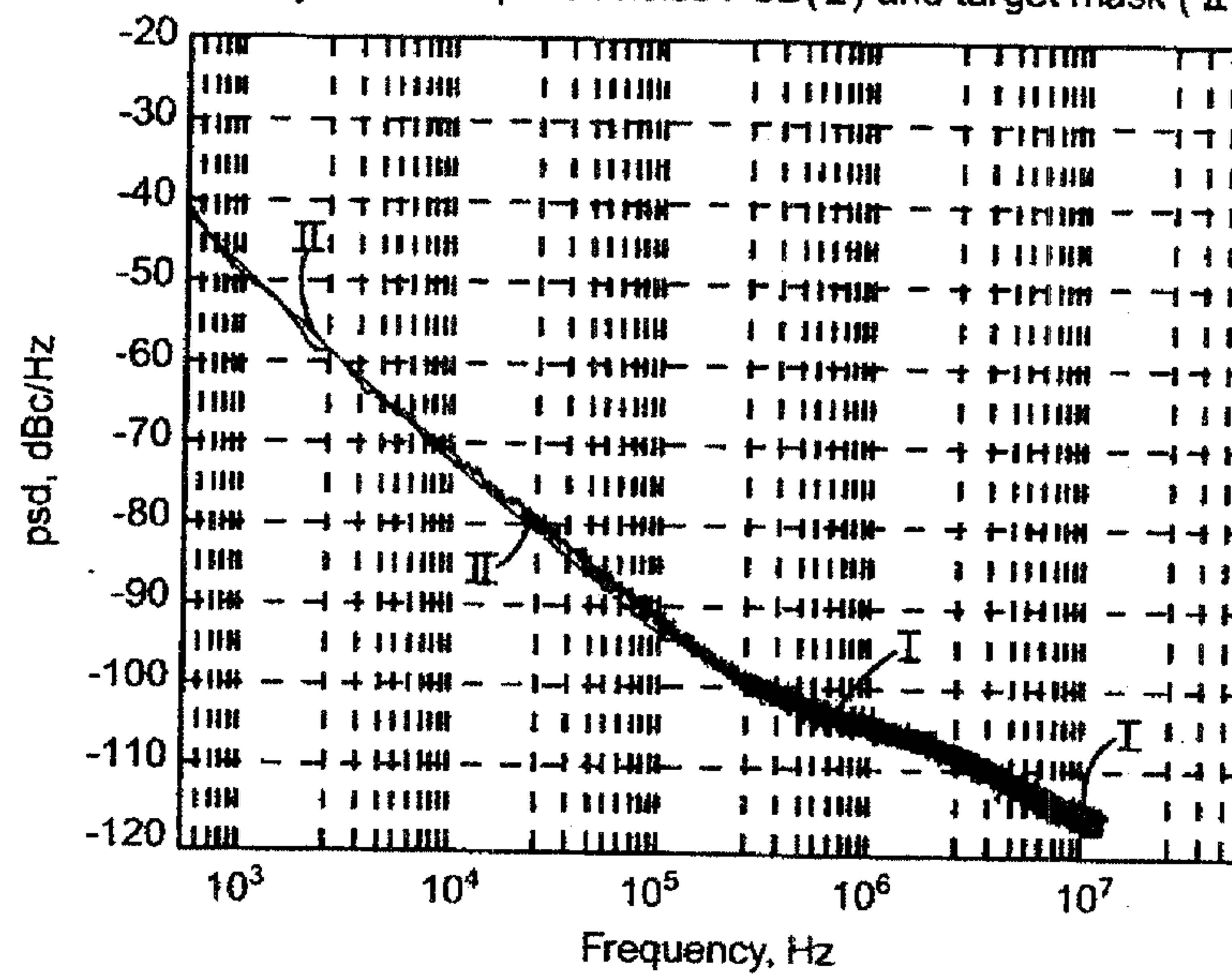
Synthesized phase noise PSD(I) and target mask (II)
