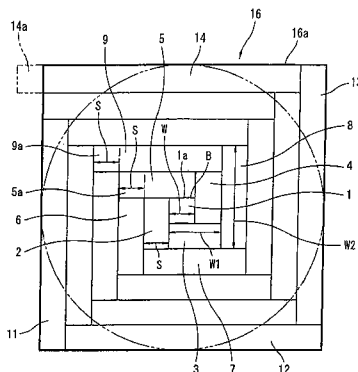
1, 21...central support section 2-14, 22-27...winding support section 16, 38, 42...square pillar 40...support unit body 41...support unit group
