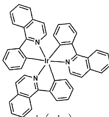
\text{Ir(piq)}_3
