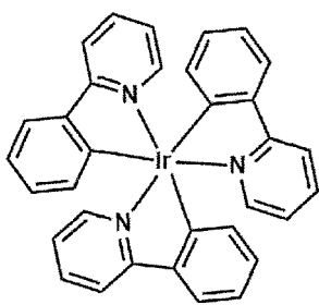
\text{Ir(ppy)}_3
