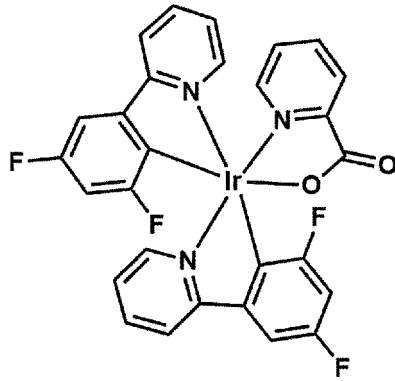
Flrpic
