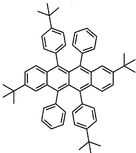
TBRb
