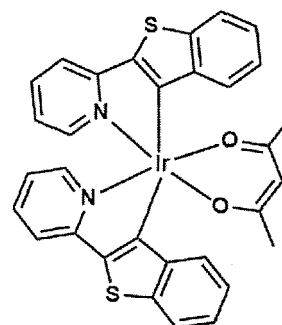
\text{Ir(btp)}_2(\text{acac})
