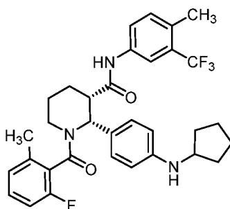
(Compound 1)
