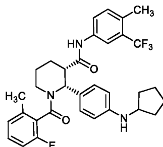
(Compound 1)
