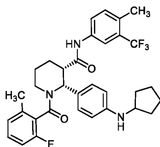
(Compound 1)
