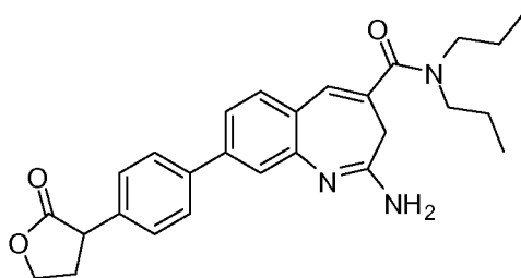
(1E,4E)-2-Amino-8-(4-(2-oxotetrahydrofuran-3-yl)phenyl)-N,N-dipropyl-3H-benzo[b]azepine-4-carboxamide
