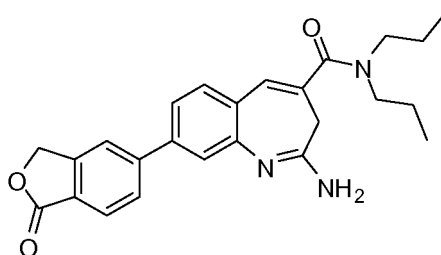
(1E,4E)-2-Amino-8-(1-oxo-1,3-dihydroisobenzofuran-5-yl)-N,N-dipropyl-3H-benzo[b]azepine-4-carboxamide
