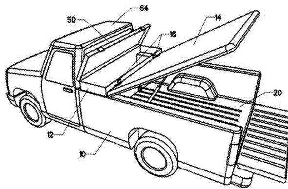
FIG. 9 PRIOR ART
