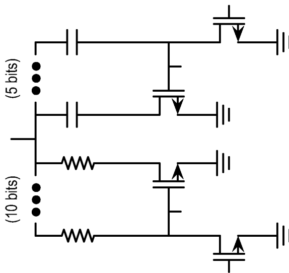
FIG. 95 small signal balancing network 880
