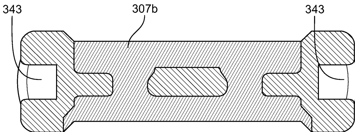
SECTION F-F
