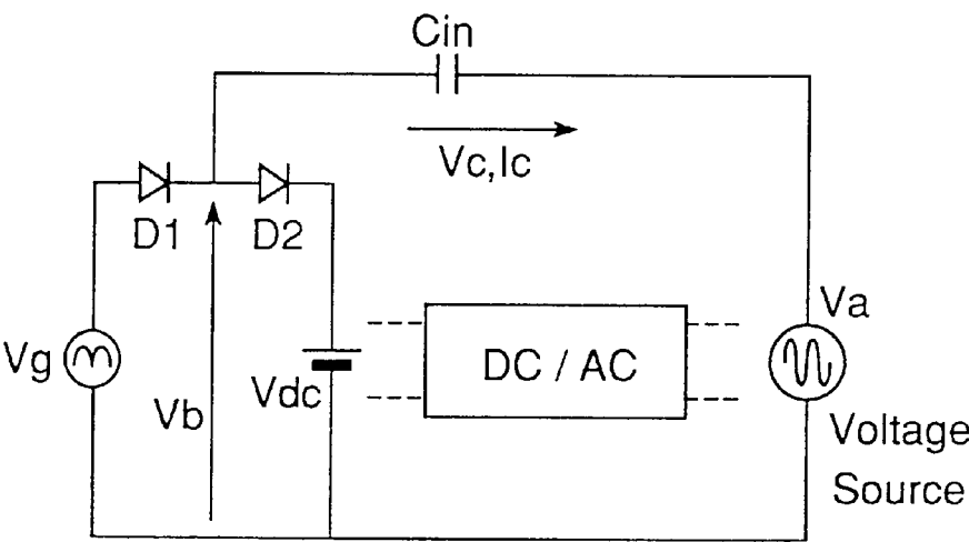
Fig.83 PRIOR ART
