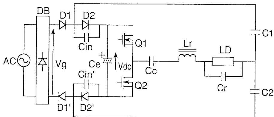
Fig.91 PRIOR ART
