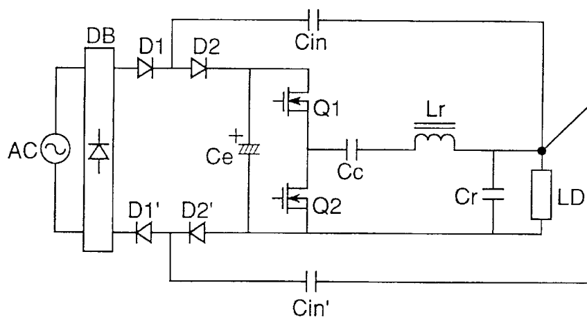
Fig.90 PRIOR ART
