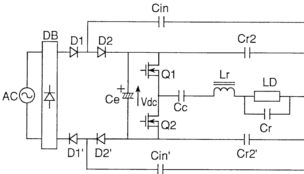
Fig.93 PRIOR ART
