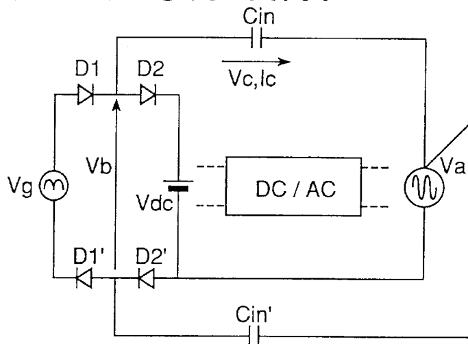
Fig.90 PRIOR ART
