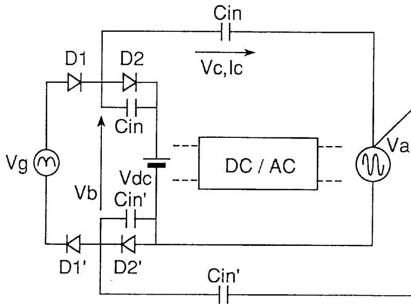
Fig.92 PRIOR ART
