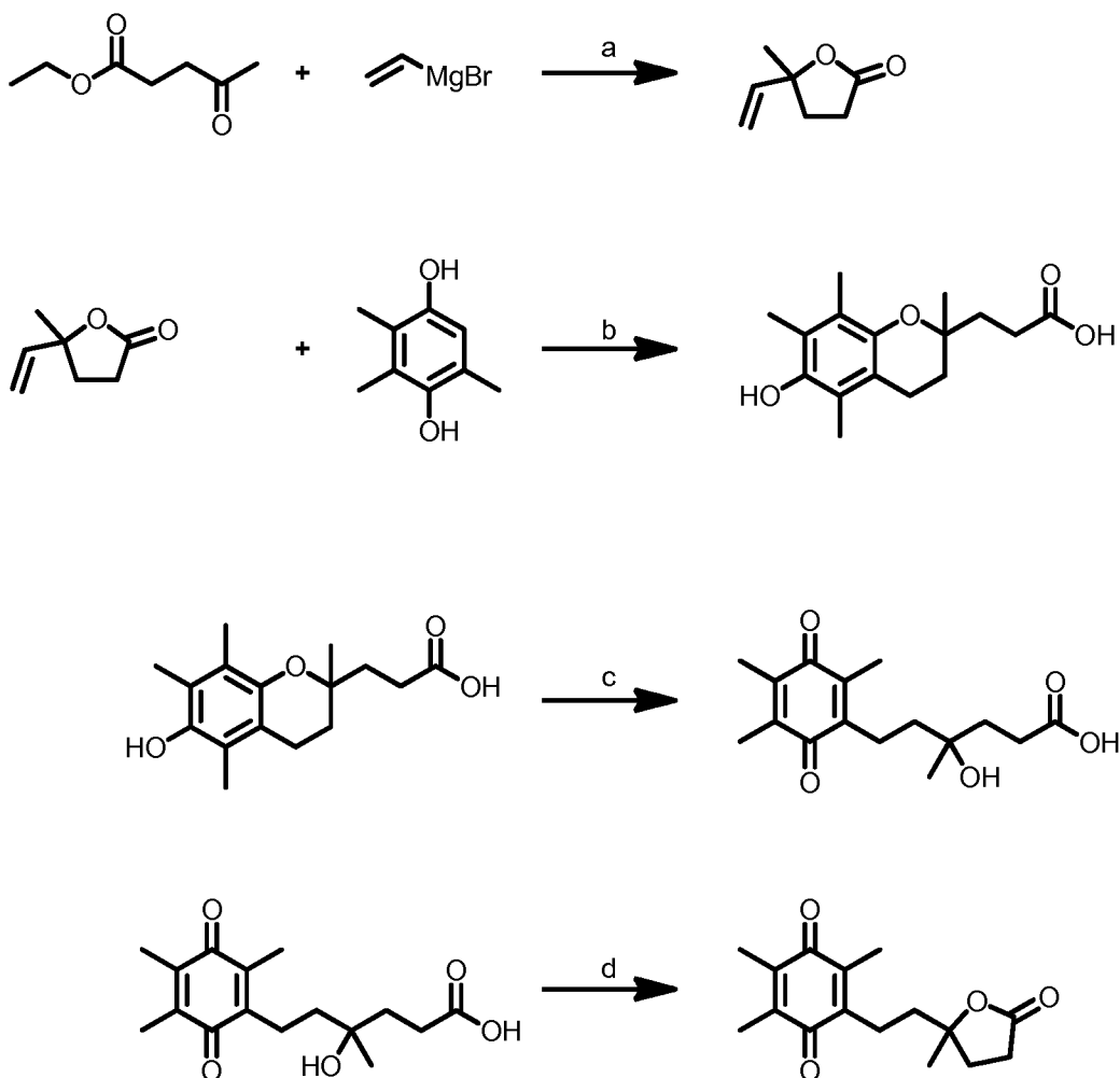
Scheme 1
