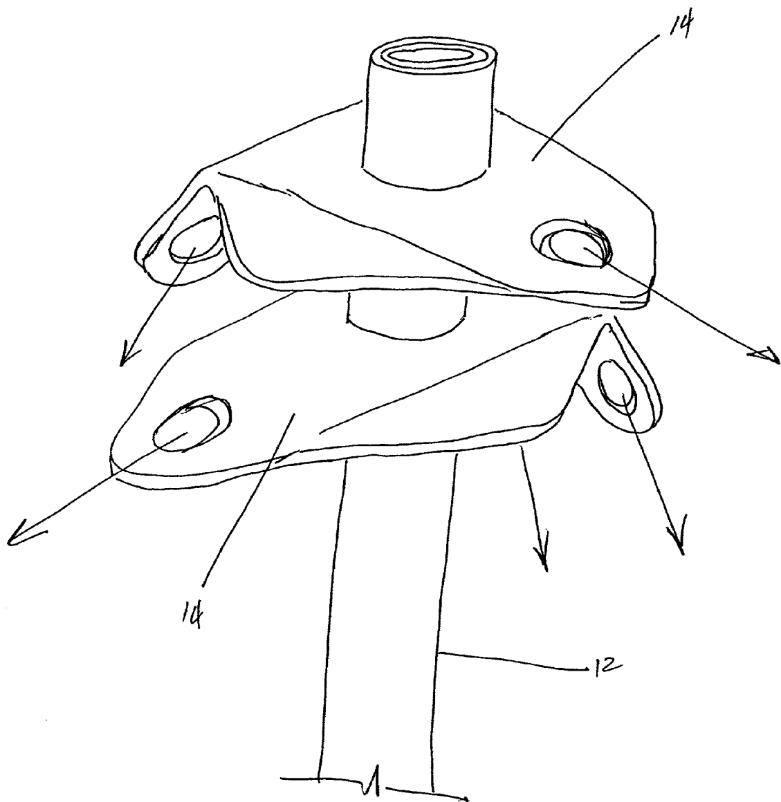
Fig 5 Quad Arrangement Roller station head,
