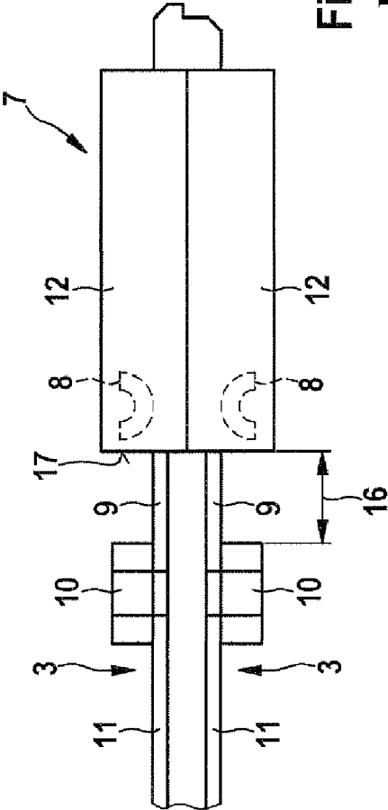
Fig. 5 Prior Art
