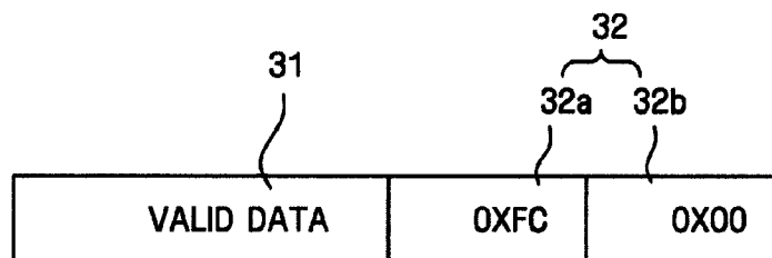
FIG. 6A (PRIOR ART)
