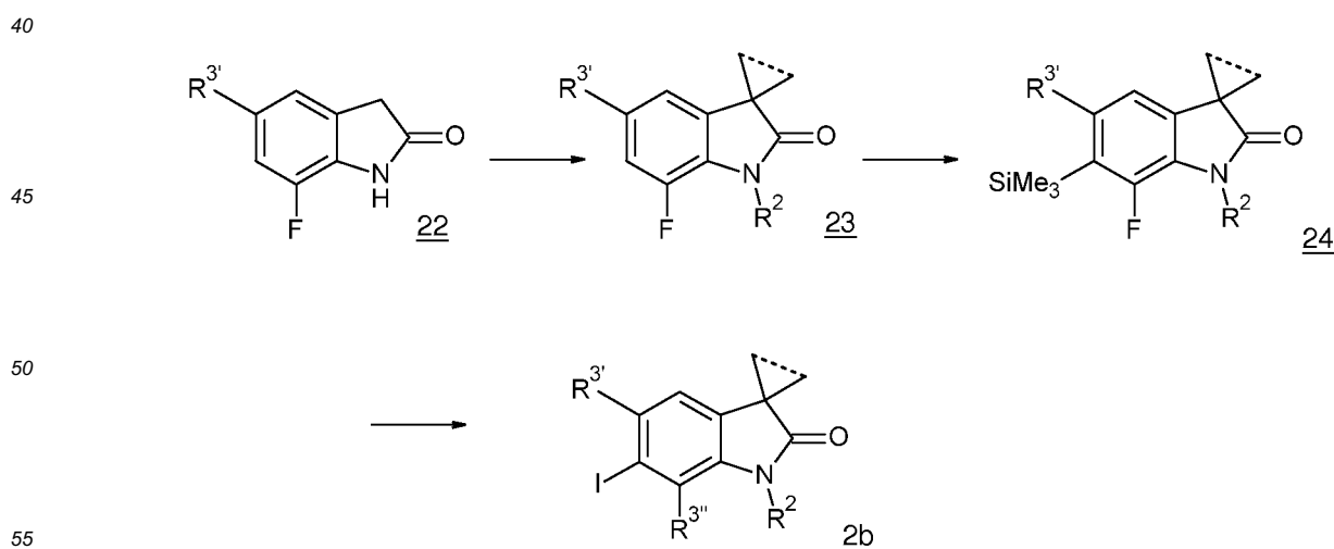
Scheme 15
