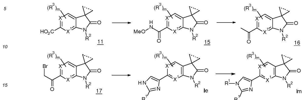
Scheme 8
