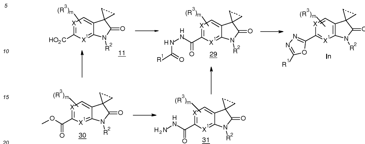
Scheme 18
