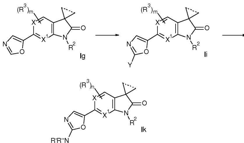
Scheme 12
