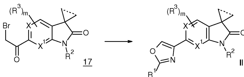
Scheme 13
