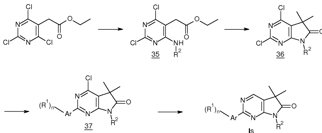
Scheme 23
