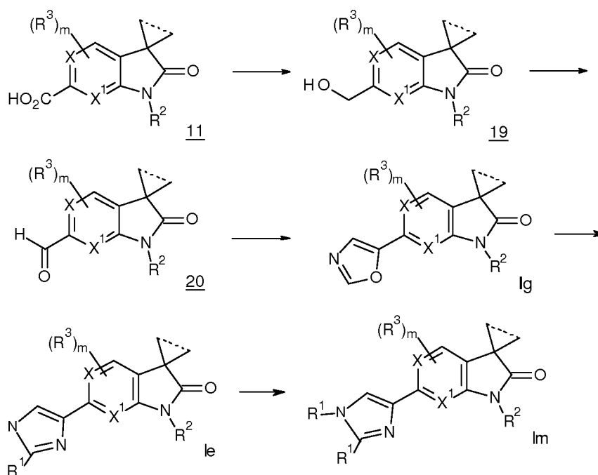
Scheme 10
