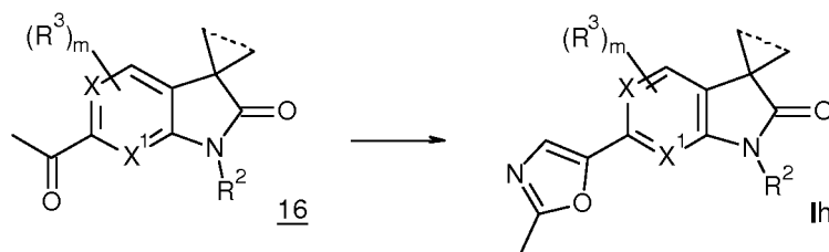
Scheme 11
