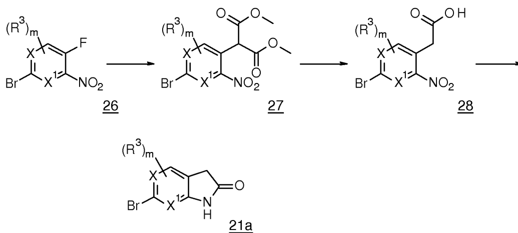
Scheme 17
