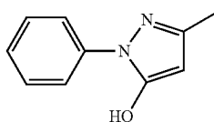
1-phenyl-3-methyl-pyrazol-5-one (comparative)
