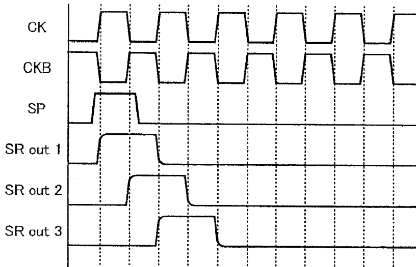
Fig. 11C Prior Art
