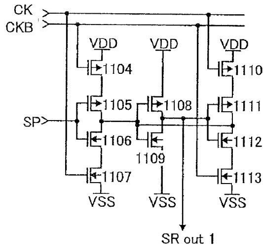
Fig. 11C Prior Art
