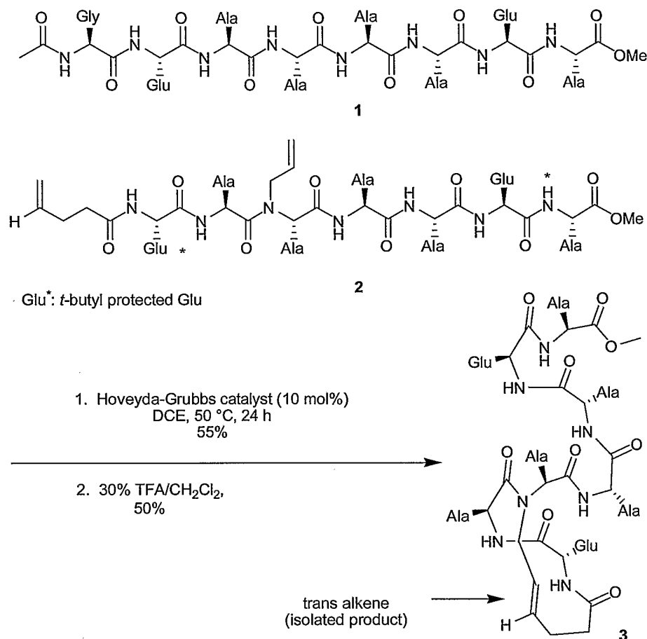
Scheme 4
