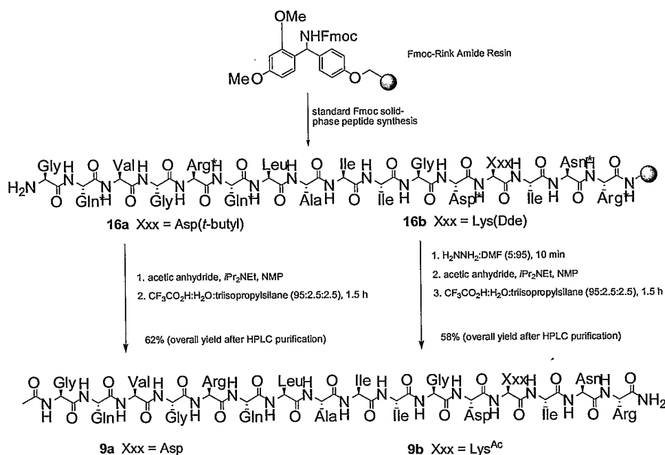
Scheme 11
