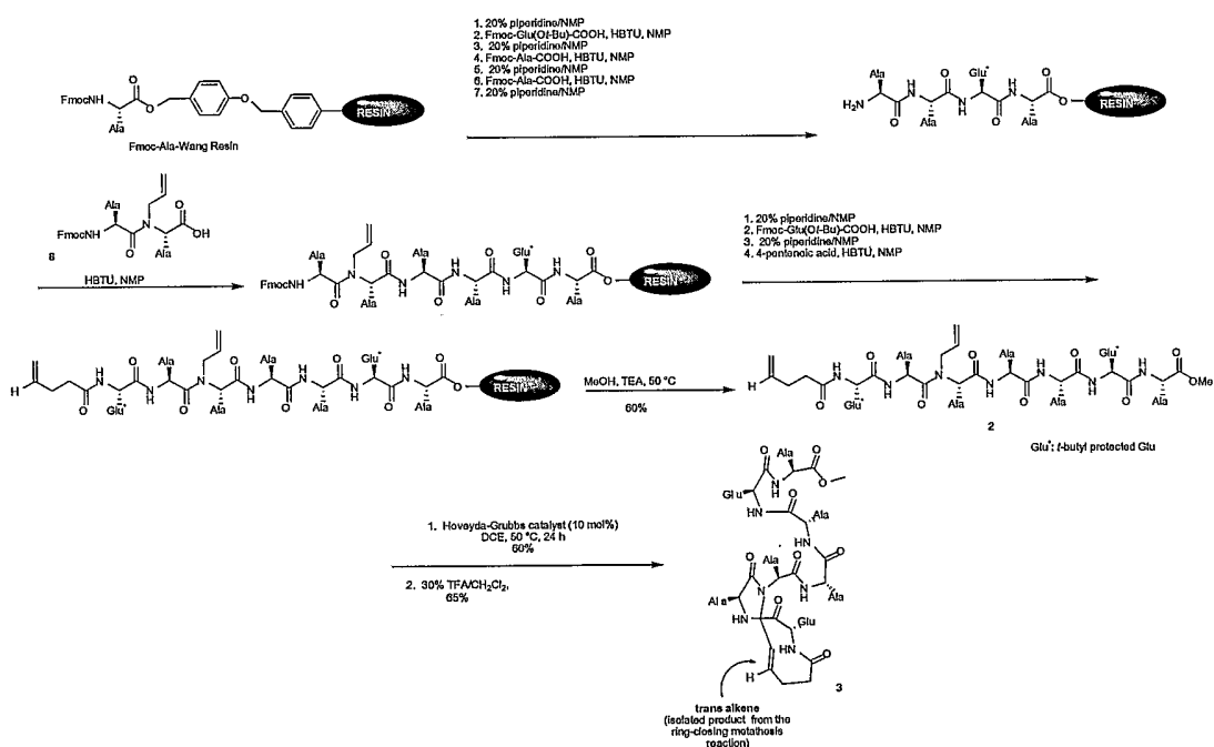
Scheme 6
