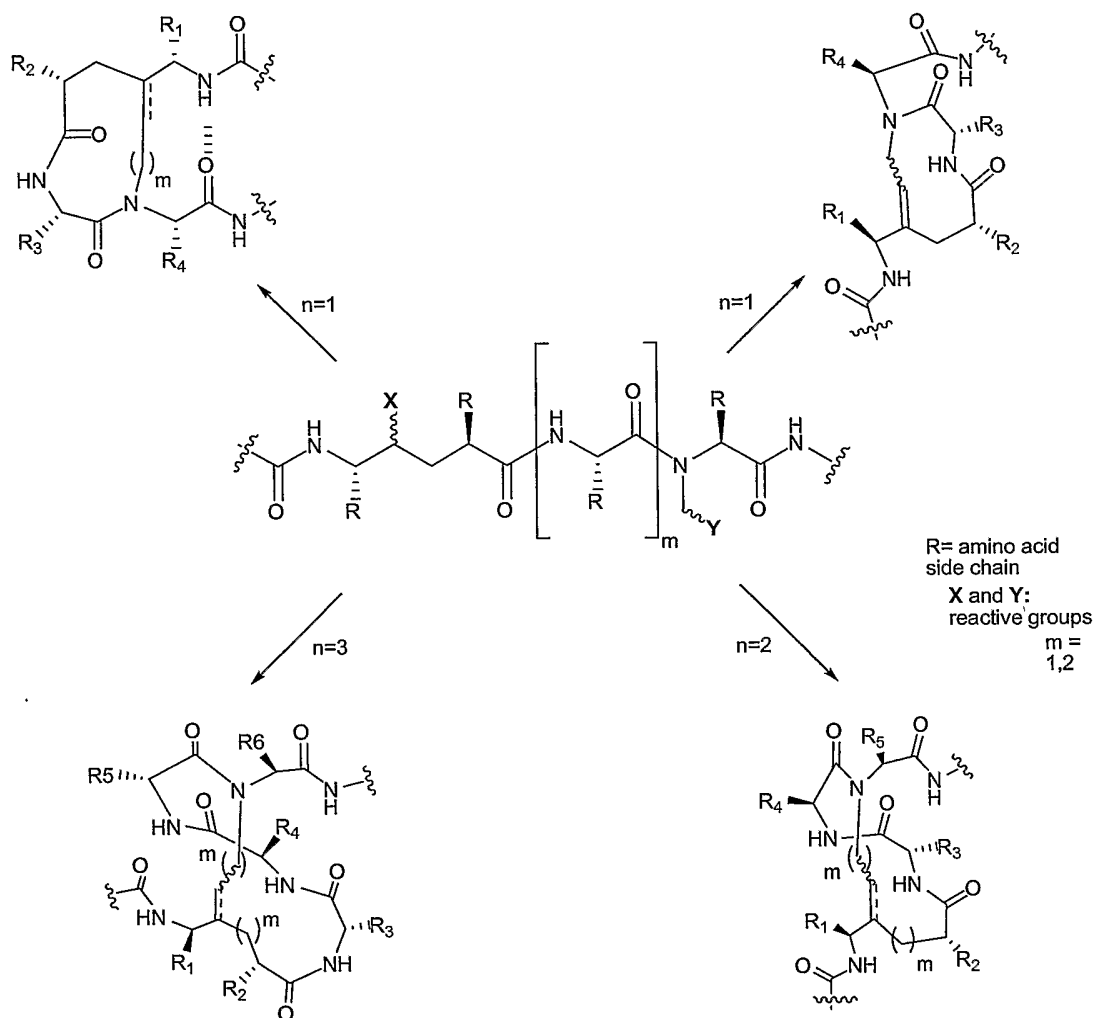
Scheme 8
