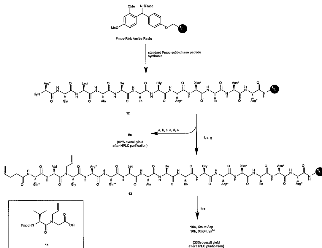
Scheme 9
