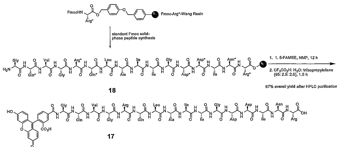
Scheme 13
