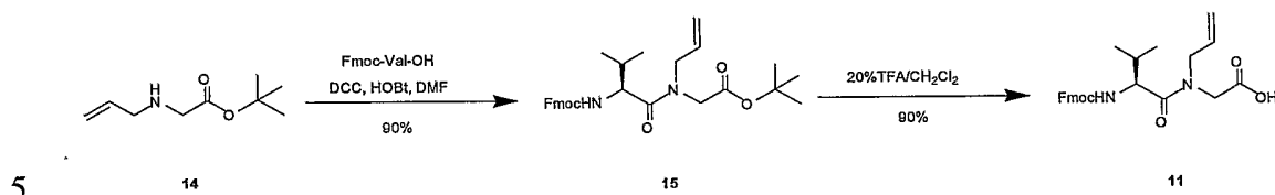
Scheme 10
