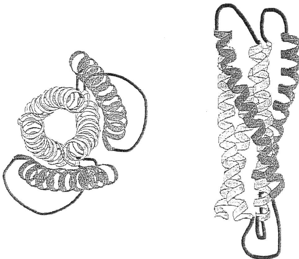
a) View from top of molecule
