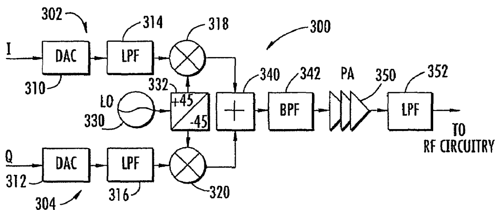
FIG. 4 (PRIOR ART)
