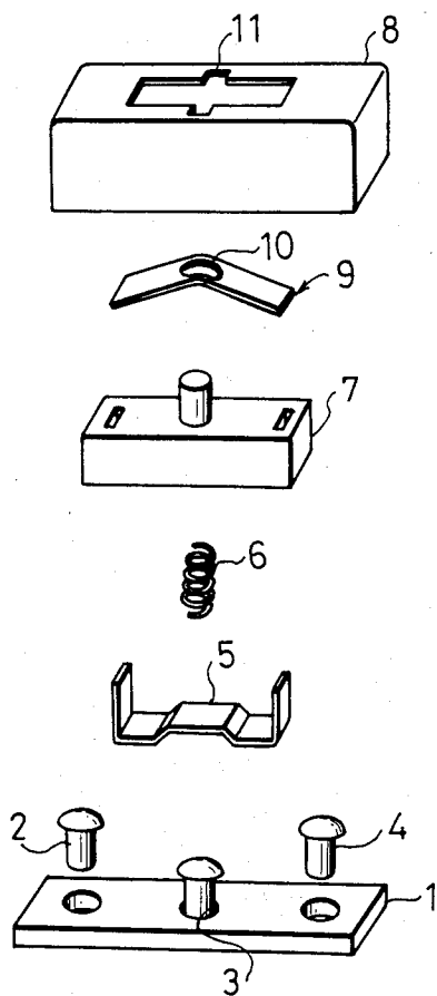
Fig.1 PRIOR ART
