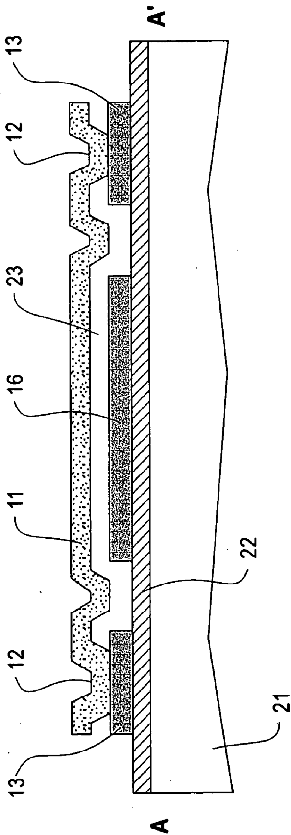
Fig. 1C Prior Art
