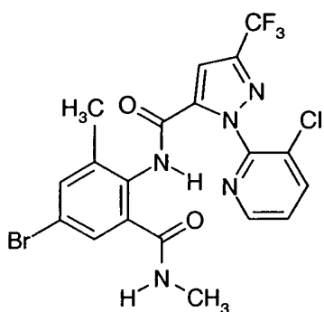
(A-2) + TX,
